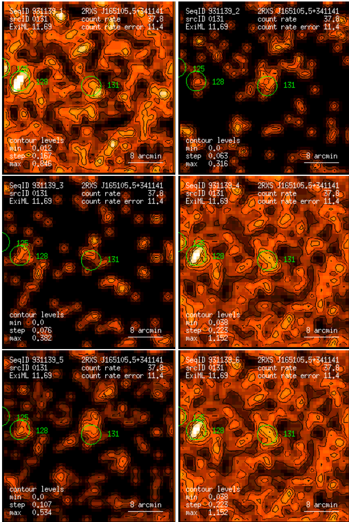
Figure 131: RASS 931139: detection 0131: band rate images, Gaussian filter: (1) PSPC channels 11 – 41, (2) 52 – 90, (3) 91 – 201, (4) 11 – 235, (5) 52 – 201, (6) 11 – 201. Broad band rates in counts/ks. Band rate contour levels in counts/ks/arcmin 2 .
