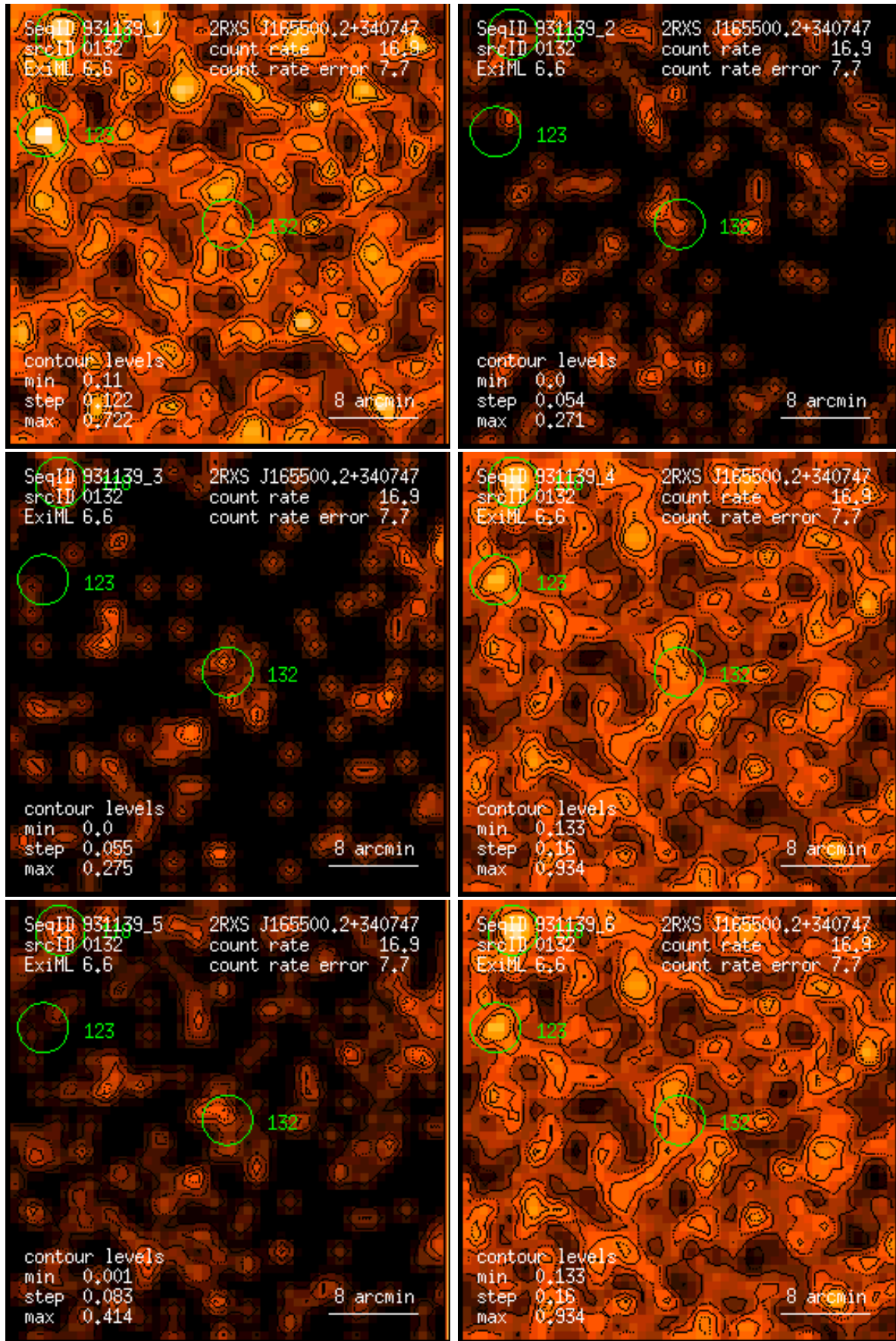
Figure 132: RASS 931139: detection 0132: band rate images, Gaussian filter: (1) PSPC channels 11 – 41, (2) 52 – 90, (3) 91 – 201, (4) 11 – 235, (5) 52 – 201, (6) 11 – 201. Broad band rates in counts/ks. Band rate contour levels in counts/ks/arcmin 2 .
