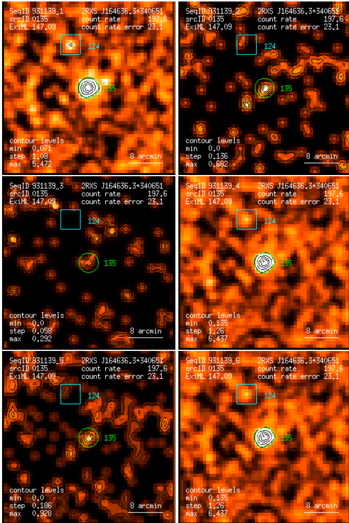
Figure 135: RASS 931139: detection 0135: band rate images, Gaussian filter: (1) PSPC channels 11 – 41, (2) 52 – 90, (3) 91 – 201, (4) 11 – 235, (5) 52 – 201, (6) 11 – 201. Broad band rates in counts/ks. Band rate contour levels in counts/ks/arcmin 2 .
