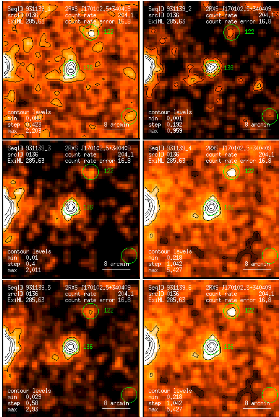
Figure 136: RASS 931139: detection 0136: band rate images, Gaussian filter: (1) PSPC channels 11 – 41, (2) 52 – 90, (3) 91 – 201, (4) 11 – 235, (5) 52 – 201, (6) 11 – 201. Broad band rates in counts/ks. Band rate contour levels in counts/ks/arcmin 2 .
