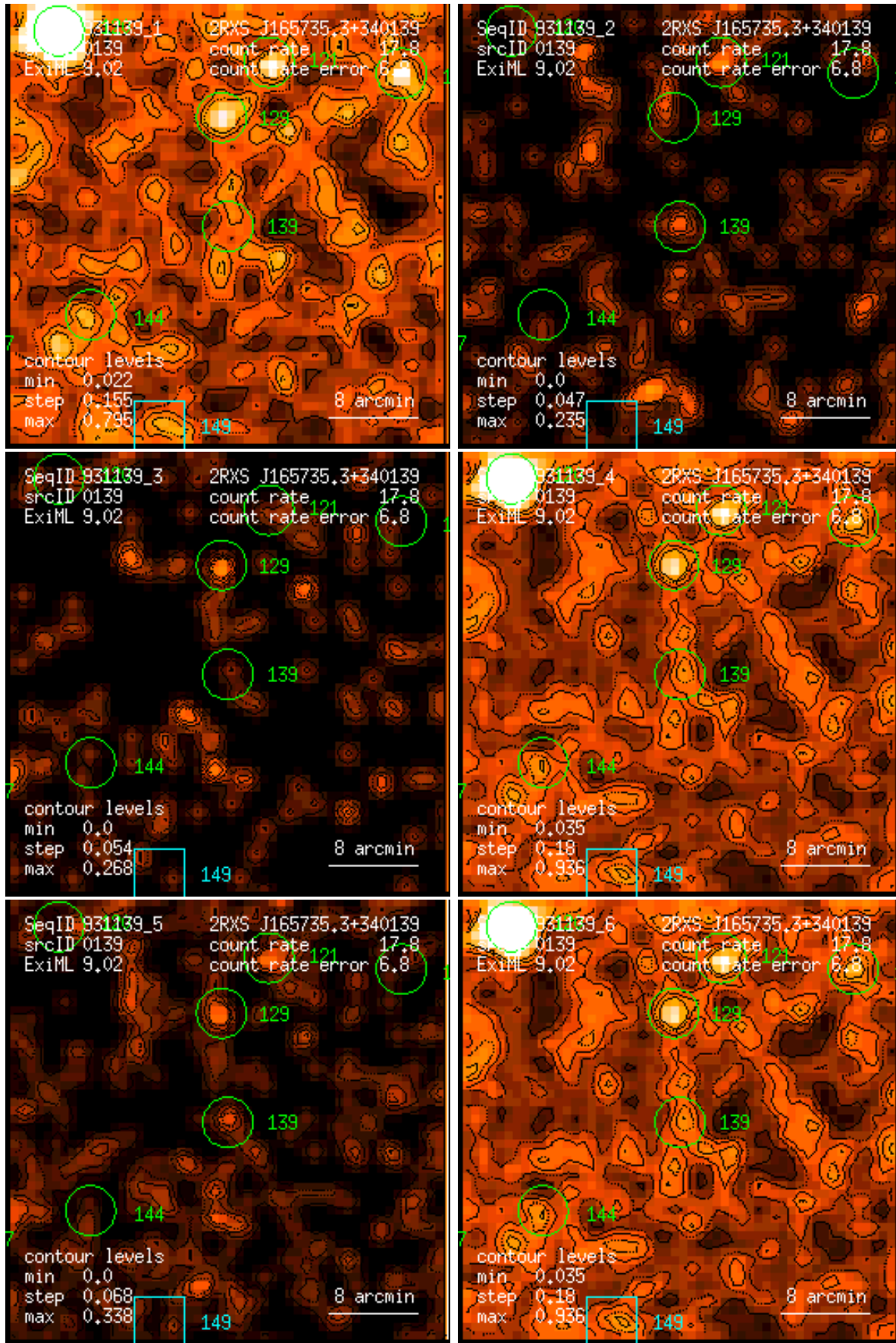
Figure 139: RASS 931139: detection 0139: band rate images, Gaussian filter: (1) PSPC channels 11 – 41, (2) 52 – 90, (3) 91 – 201, (4) 11 – 235, (5) 52 – 201, (6) 11 – 201. Broad band rates in counts/ks. Band rate contour levels in counts/ks/arcmin 2 .
