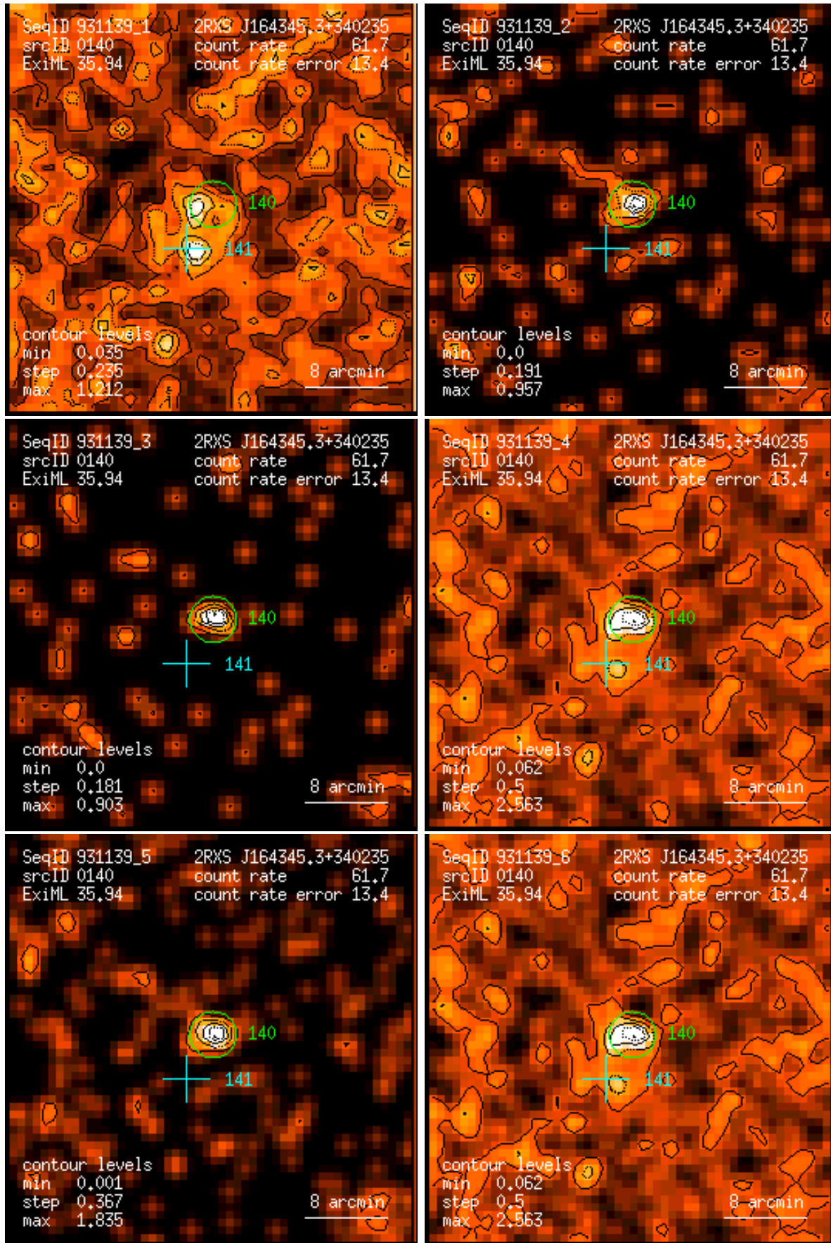
Figure 140: RASS 931139: detection 0140: band rate images, Gaussian filter: (1) PSPC channels 11 – 41, (2) 52 – 90, (3) 91 – 201, (4) 11 – 235, (5) 52 – 201, (6) 11 – 201. Broad band rates in counts/ks. Band rate contour levels in counts/ks/arcmin 2 .
