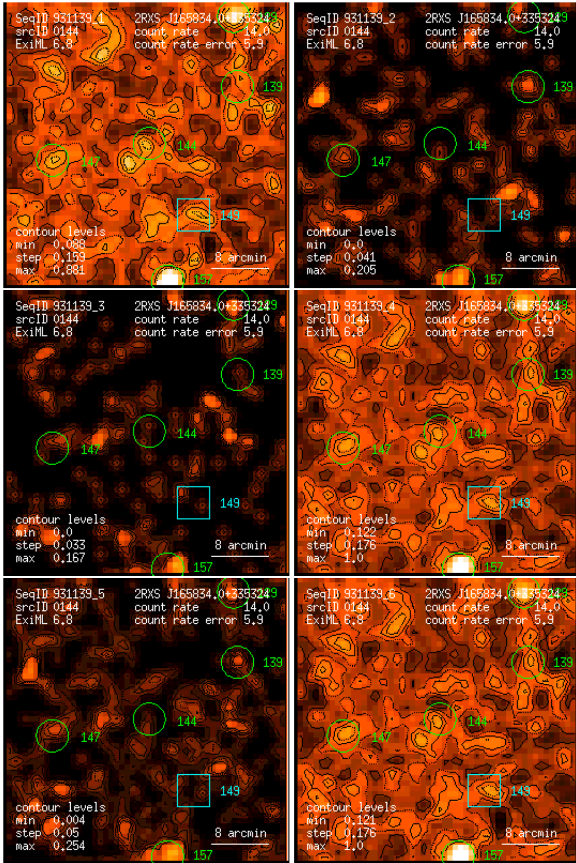
Figure 144: RASS 931139: detection 0144: band rate images, Gaussian filter: (1) PSPC channels 11 – 41, (2) 52 – 90, (3) 91 – 201, (4) 11 – 235, (5) 52 – 201, (6) 11 – 201. Broad band rates in counts/ks. Band rate contour levels in counts/ks/arcmin 2 .
