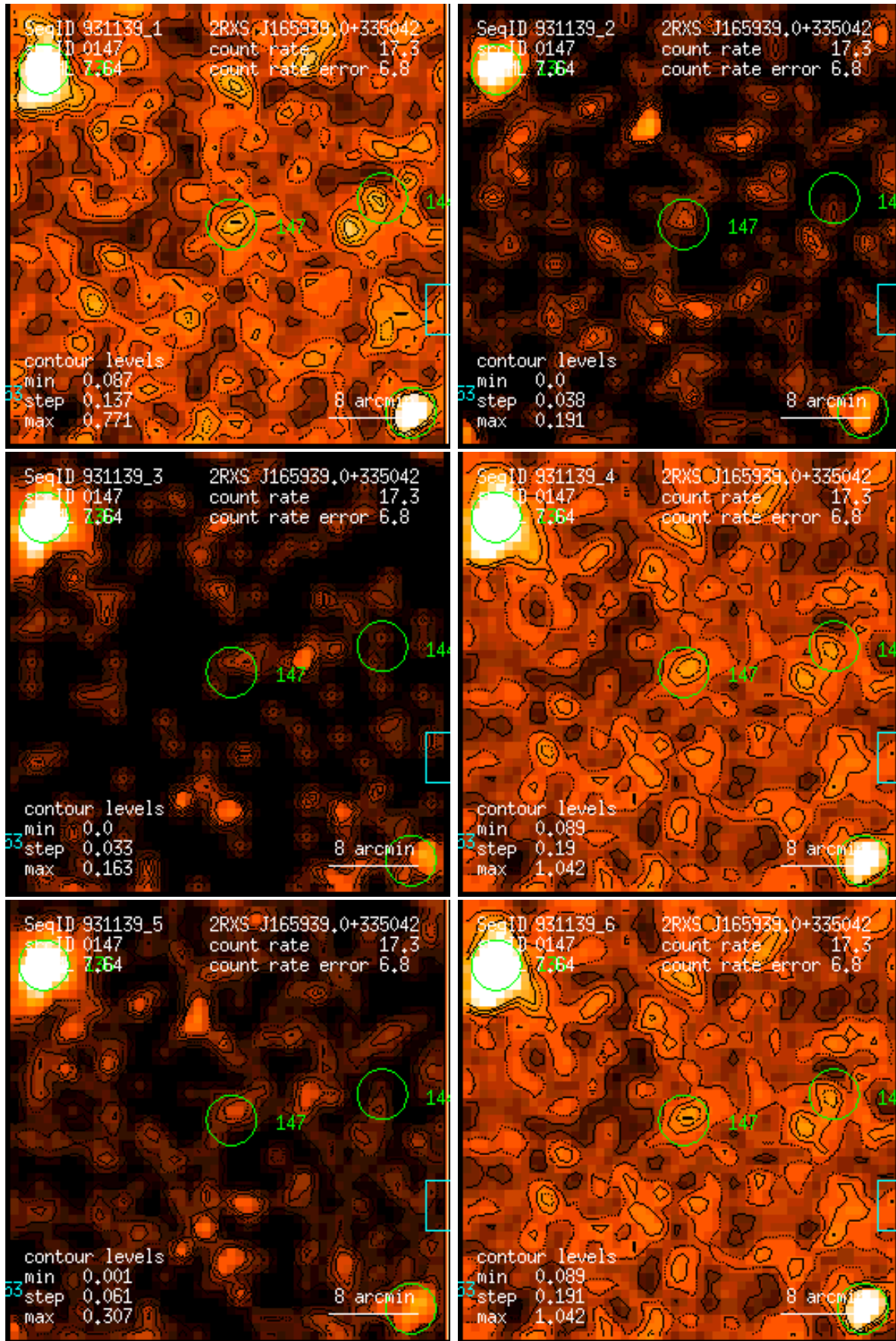
Figure 147: RASS 931139: detection 0147: band rate images, Gaussian filter: (1) PSPC channels 11 – 41, (2) 52 – 90, (3) 91 – 201, (4) 11 – 235, (5) 52 – 201, (6) 11 – 201. Broad band rates in counts/ks. Band rate contour levels in counts/ks/arcmin 2 .
