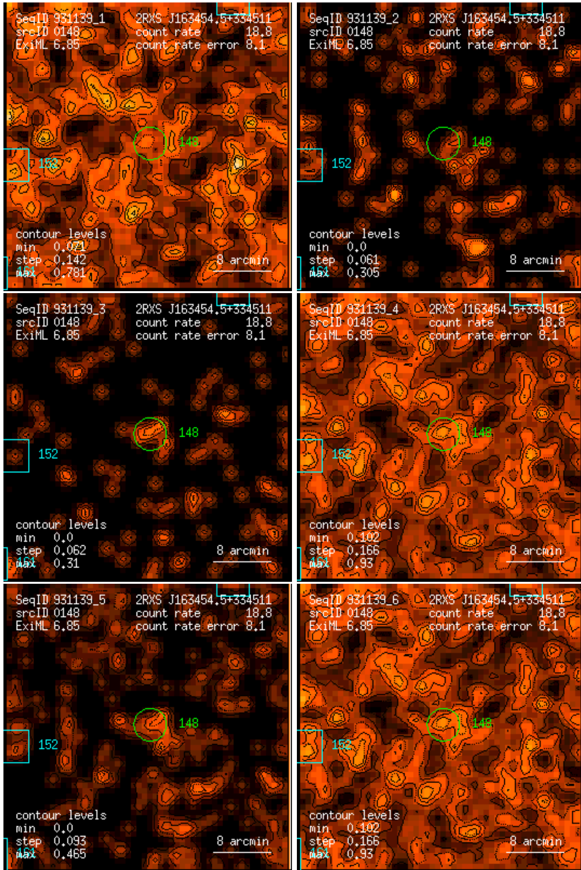
Figure 148: RASS 931139: detection 0148: band rate images, Gaussian filter: (1) PSPC channels 11 – 41, (2) 52 – 90, (3) 91 – 201, (4) 11 – 235, (5) 52 – 201, (6) 11 – 201. Broad band rates in counts/ks. Band rate contour levels in counts/ks/arcmin 2 .
