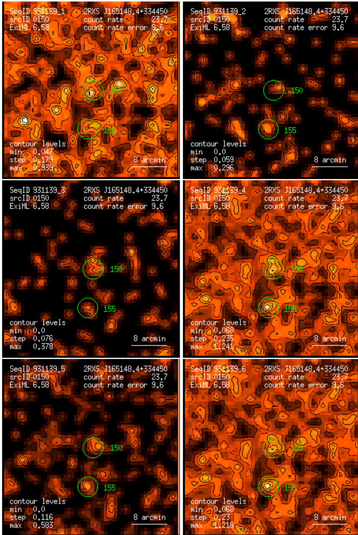
Figure 150: RASS 931139: detection 0150: band rate images, Gaussian filter: (1) PSPC channels 11 – 41, (2) 52 – 90, (3) 91 – 201, (4) 11 – 235, (5) 52 – 201, (6) 11 – 201. Broad band rates in counts/ks. Band rate contour levels in counts/ks/arcmin 2 .
