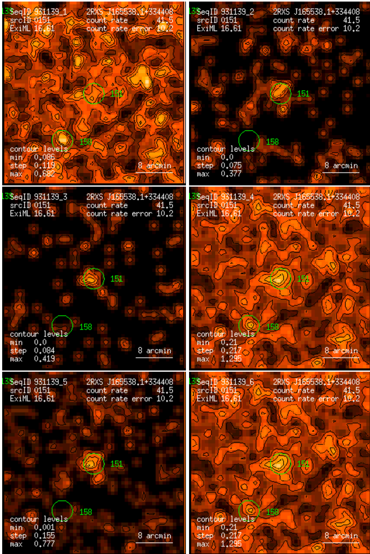
Figure 151: RASS 931139: detection 0151: band rate images, Gaussian filter: (1) PSPC channels 11 – 41, (2) 52 – 90, (3) 91 – 201, (4) 11 – 235, (5) 52 – 201, (6) 11 – 201. Broad band rates in counts/ks. Band rate contour levels in counts/ks/arcmin 2 .
