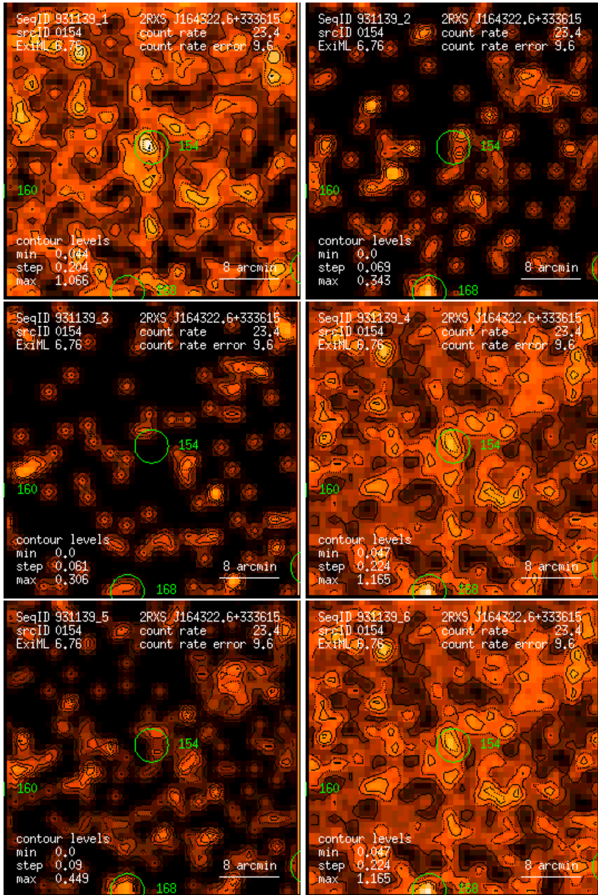
Figure 154: RASS 931139: detection 0154: band rate images, Gaussian filter: (1) PSPC channels 11 – 41, (2) 52 – 90, (3) 91 – 201, (4) 11 – 235, (5) 52 – 201, (6) 11 – 201. Broad band rates in counts/ks. Band rate contour levels in counts/ks/arcmin 2 .
