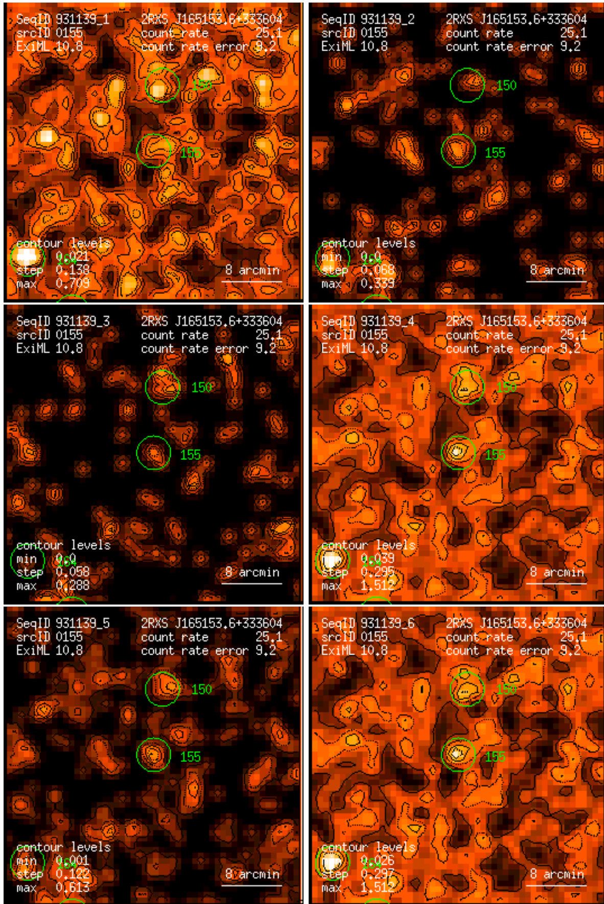
Figure 155: RASS 931139: detection 0155: band rate images, Gaussian filter: (1) PSPC channels 11 – 41, (2) 52 – 90, (3) 91 – 201, (4) 11 – 235, (5) 52 – 201, (6) 11 – 201. Broad band rates in counts/ks. Band rate contour levels in counts/ks/arcmin 2 .
