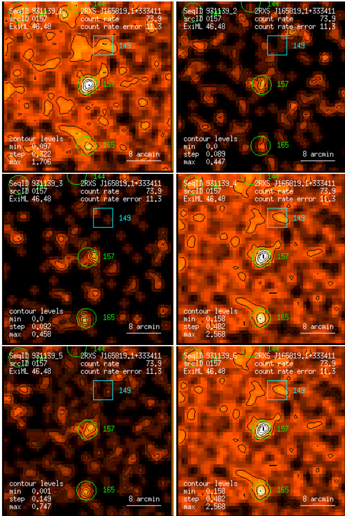
Figure 157: RASS 931139: detection 0157: band rate images, Gaussian filter: (1) PSPC channels 11 – 41, (2) 52 – 90, (3) 91 – 201, (4) 11 – 235, (5) 52 – 201, (6) 11 – 201. Broad band rates in counts/ks. Band rate contour levels in counts/ks/arcmin 2 .
