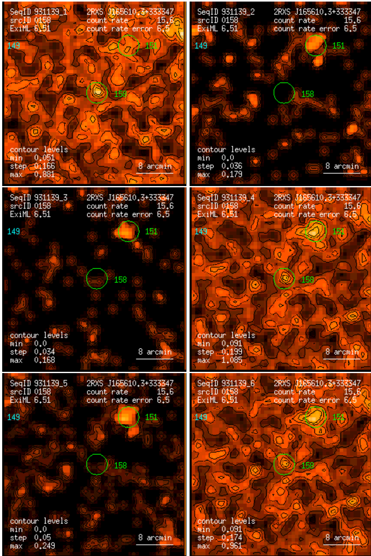
Figure 158: RASS 931139: detection 0158: band rate images, Gaussian filter: (1) PSPC channels 11 – 41, (2) 52 – 90, (3) 91 – 201, (4) 11 – 235, (5) 52 – 201, (6) 11 – 201. Broad band rates in counts/ks. Band rate contour levels in counts/ks/arcmin 2 .
