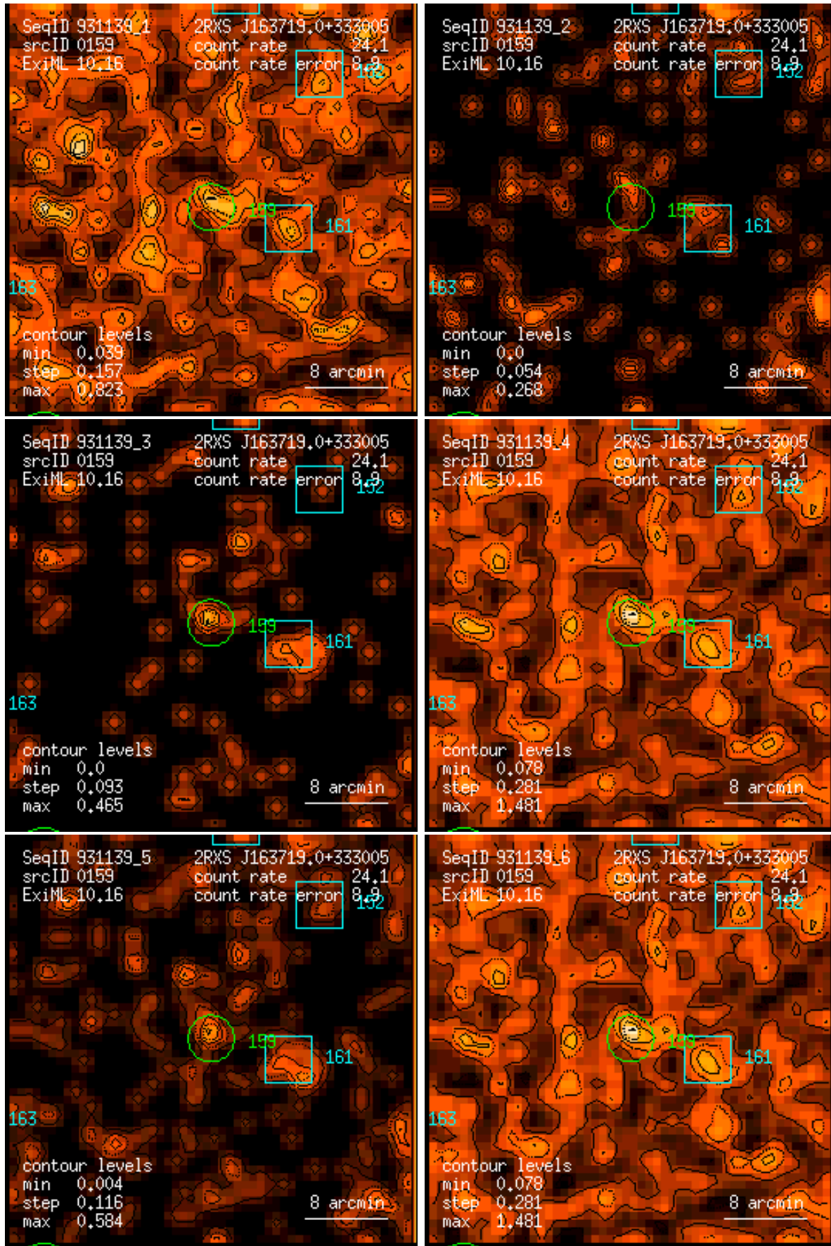
Figure 159: RASS 931139: detection 0159: band rate images, Gaussian filter: (1) PSPC channels 11 – 41, (2) 52 – 90, (3) 91 – 201, (4) 11 – 235, (5) 52 – 201, (6) 11 – 201. Broad band rates in counts/ks. Band rate contour levels in counts/ks/arcmin 2 .
