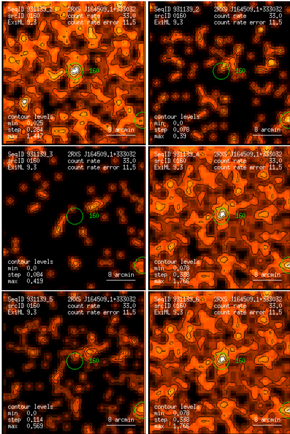
Figure 160: RASS 931139: detection 0160: band rate images, Gaussian filter: (1) PSPC channels 11 – 41, (2) 52 – 90, (3) 91 – 201, (4) 11 – 235, (5) 52 – 201, (6) 11 – 201. Broad band rates in counts/ks. Band rate contour levels in counts/ks/arcmin 2 .
