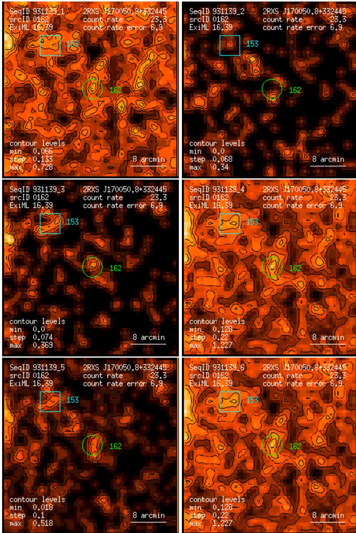
Figure 162: RASS 931139: detection 0162: band rate images, Gaussian filter: (1) PSPC channels 11 – 41, (2) 52 – 90, (3) 91 – 201, (4) 11 – 235, (5) 52 – 201, (6) 11 – 201. Broad band rates in counts/ks. Band rate contour levels in counts/ks/arcmin 2 .
