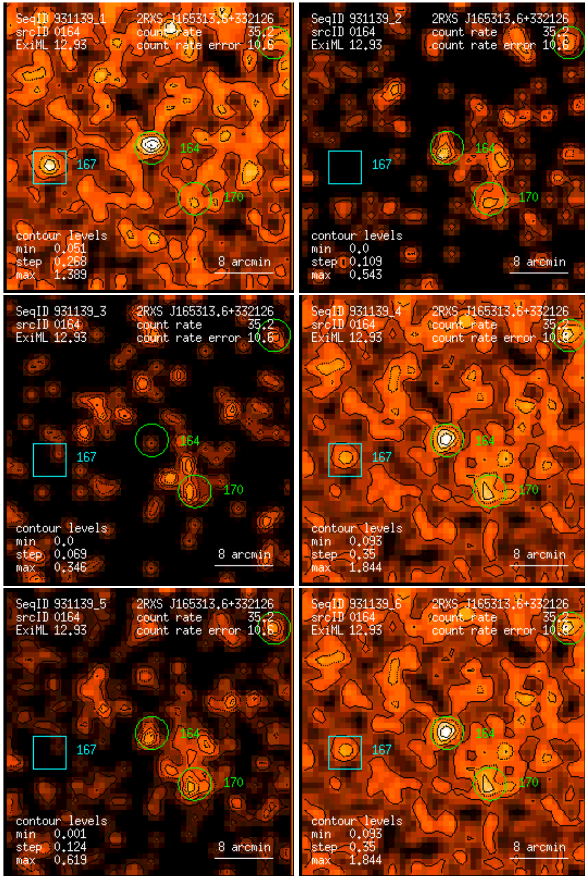
Figure 164: RASS 931139: detection 0164: band rate images, Gaussian filter: (1) PSPC channels 11 – 41, (2) 52 – 90, (3) 91 – 201, (4) 11 – 235, (5) 52 – 201, (6) 11 – 201. Broad band rates in counts/ks. Band rate contour levels in counts/ks/arcmin 2 .
