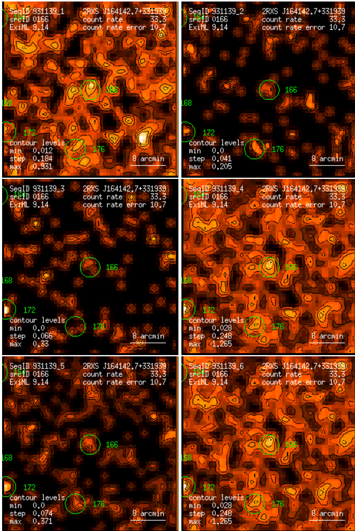
Figure 166: RASS 931139: detection 0166: band rate images, Gaussian filter: (1) PSPC channels 11 – 41, (2) 52 – 90, (3) 91 – 201, (4) 11 – 235, (5) 52 – 201, (6) 11 – 201. Broad band rates in counts/ks. Band rate contour levels in counts/ks/arcmin 2 .
