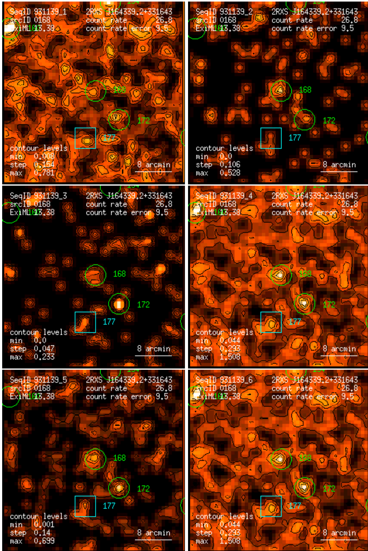
Figure 168: RASS 931139: detection 0168: band rate images, Gaussian filter: (1) PSPC channels 11 – 41, (2) 52 – 90, (3) 91 – 201, (4) 11 – 235, (5) 52 – 201, (6) 11 – 201. Broad band rates in counts/ks. Band rate contour levels in counts/ks/arcmin 2 .
