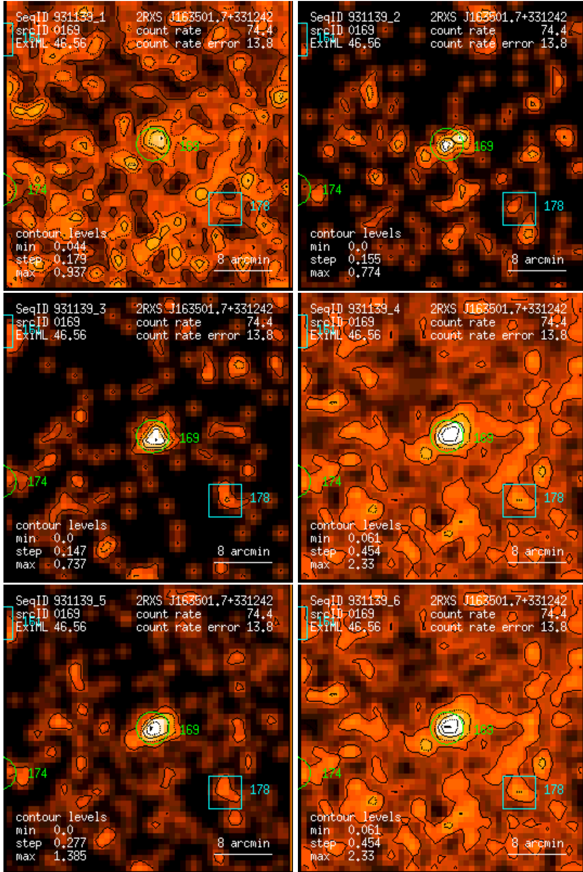
Figure 169: RASS 931139: detection 0169: band rate images, Gaussian filter: (1) PSPC channels 11 – 41, (2) 52 – 90, (3) 91 – 201, (4) 11 – 235, (5) 52 – 201, (6) 11 – 201. Broad band rates in counts/ks. Band rate contour levels in counts/ks/arcmin 2 .
