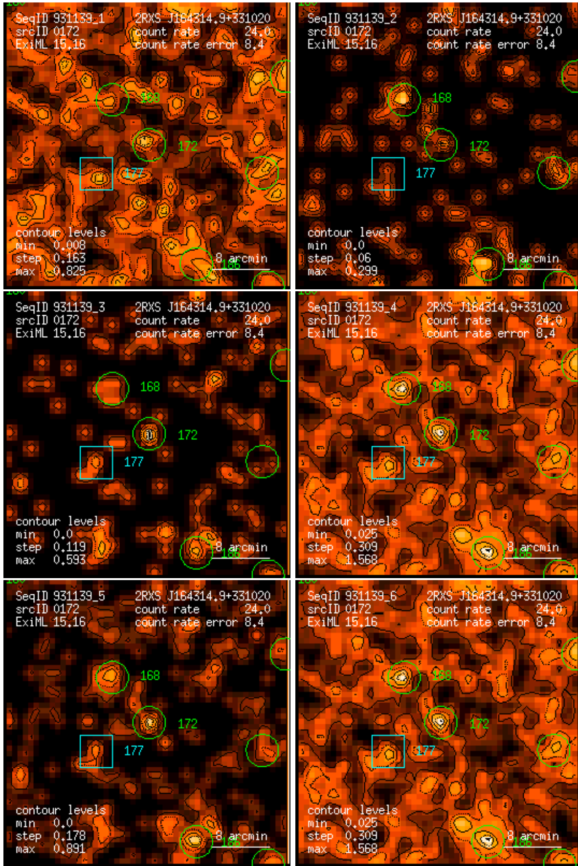
Figure 172: RASS 931139: detection 0172: band rate images, Gaussian filter: (1) PSPC channels 11 – 41, (2) 52 – 90, (3) 91 – 201, (4) 11 – 235, (5) 52 – 201, (6) 11 – 201. Broad band rates in counts/ks. Band rate contour levels in counts/ks/arcmin 2 .
