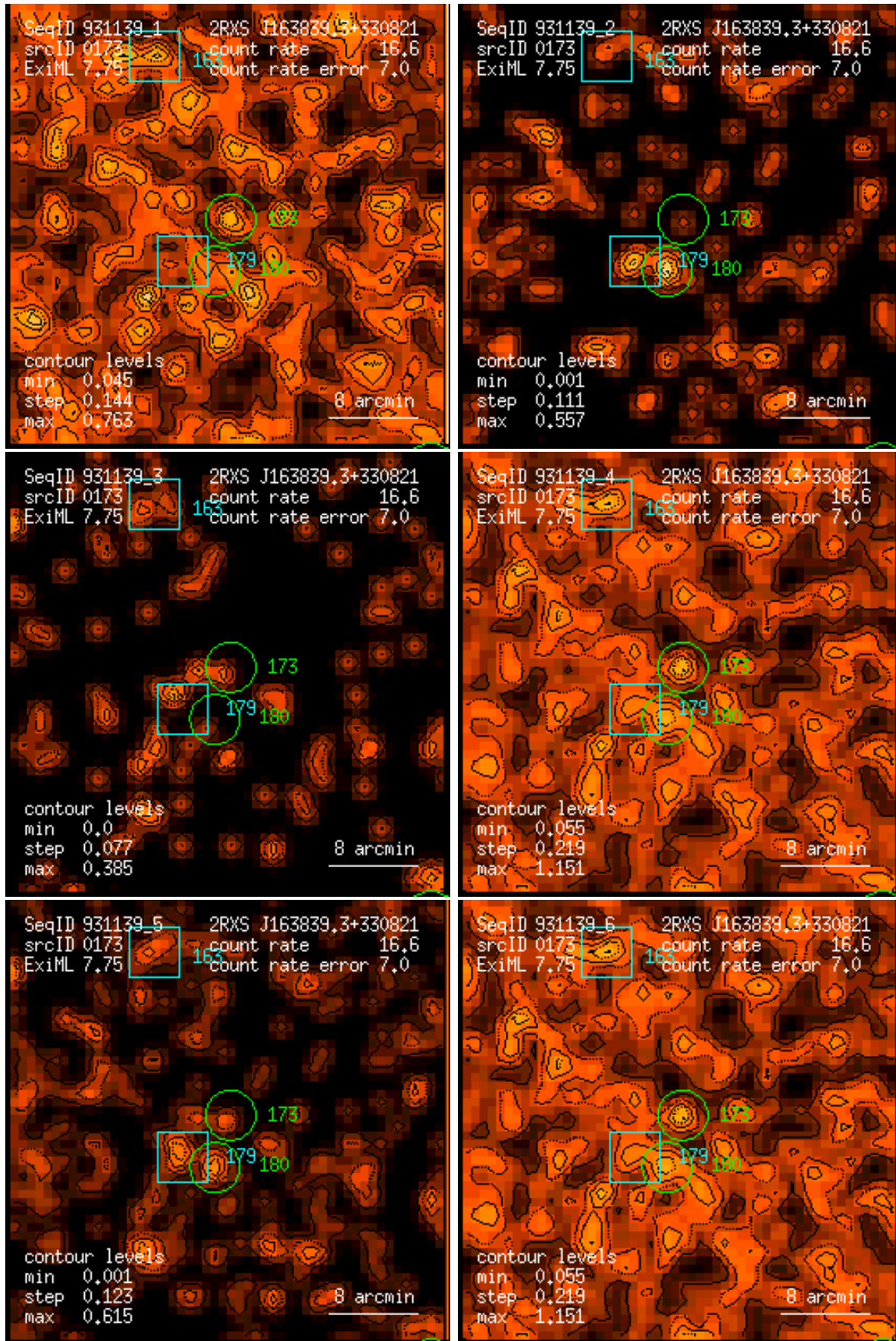
Figure 173: RASS 931139: detection 0173: band rate images, Gaussian filter: (1) PSPC channels 11 – 41, (2) 52 – 90, (3) 91 – 201, (4) 11 – 235, (5) 52 – 201, (6) 11 – 201. Broad band rates in counts/ks. Band rate contour levels in counts/ks/arcmin 2 .
