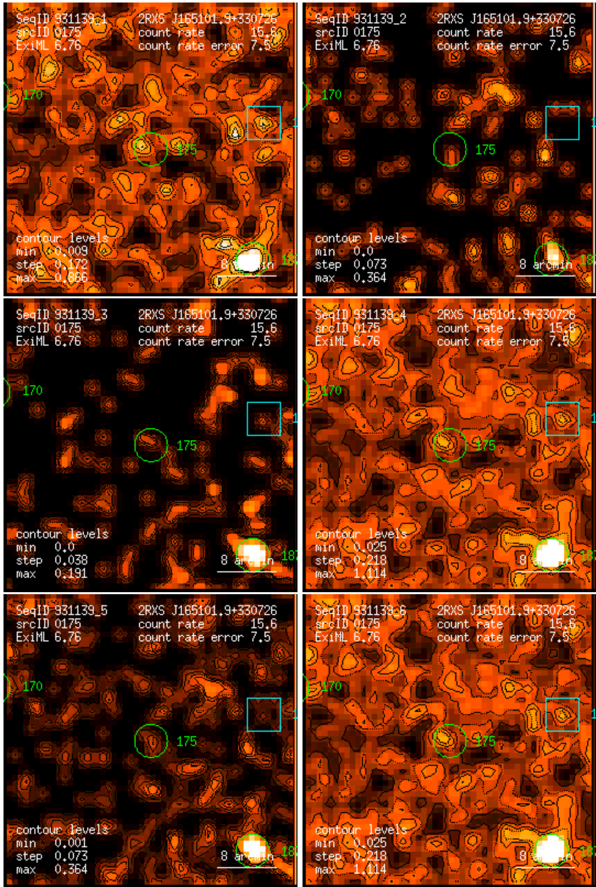
Figure 175: RASS 931139: detection 0175: band rate images, Gaussian filter: (1) PSPC channels 11 – 41, (2) 52 – 90, (3) 91 – 201, (4) 11 – 235, (5) 52 – 201, (6) 11 – 201. Broad band rates in counts/ks. Band rate contour levels in counts/ks/arcmin 2 .
