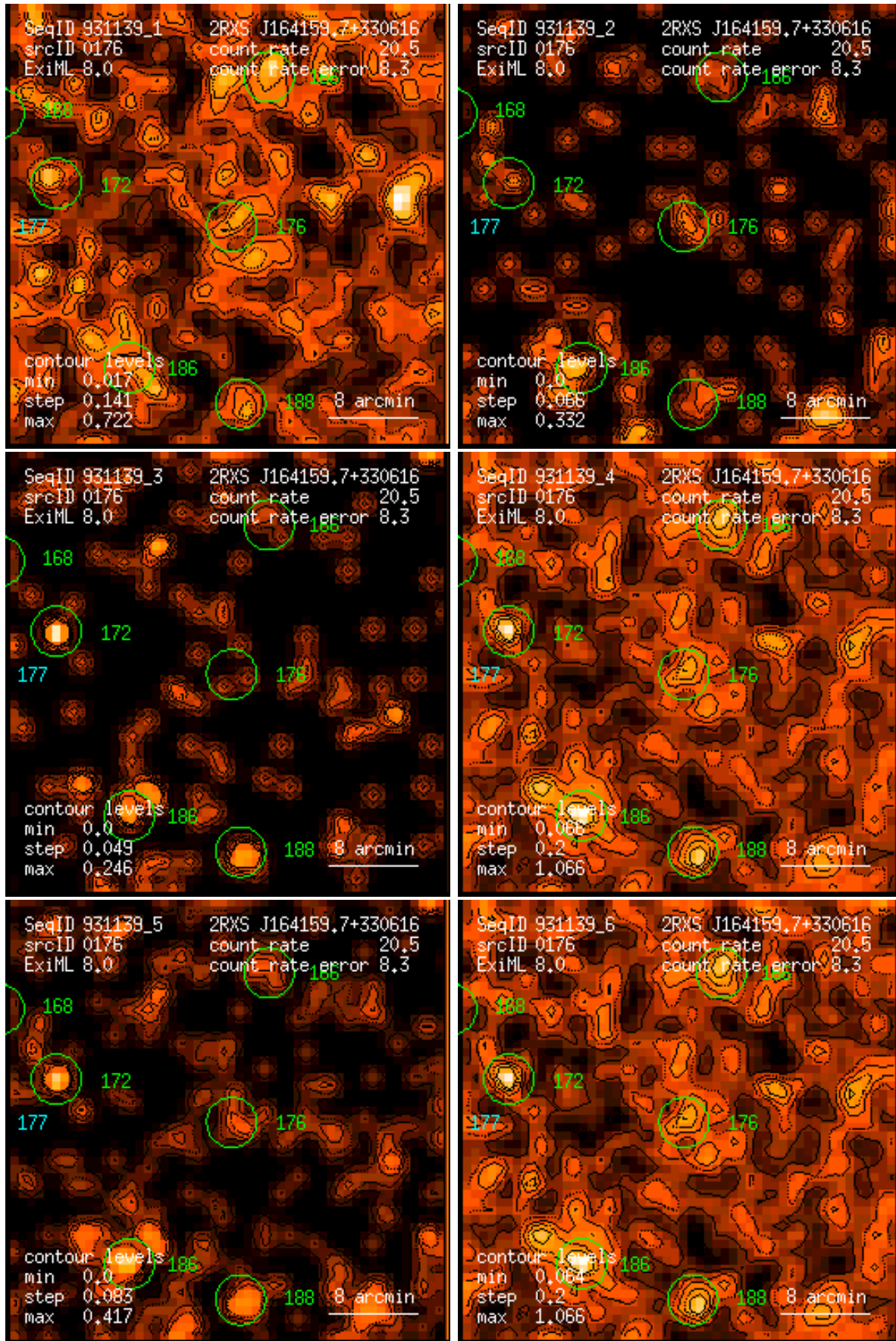
Figure 176: RASS 931139: detection 0176: band rate images, Gaussian filter: (1) PSPC channels 11 – 41, (2) 52 – 90, (3) 91 – 201, (4) 11 – 235, (5) 52 – 201, (6) 11 – 201. Broad band rates in counts/ks. Band rate contour levels in counts/ks/arcmin 2 .
