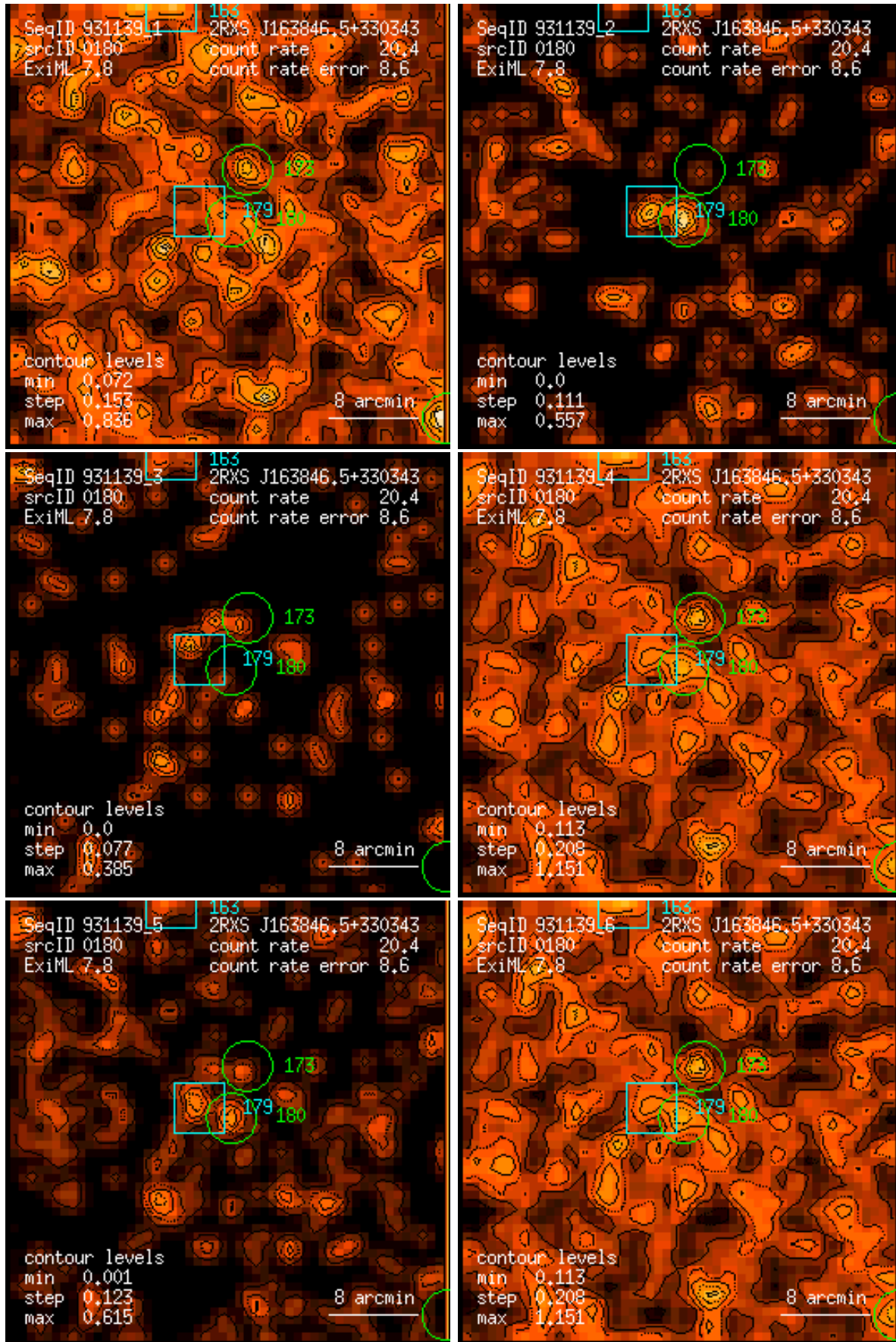
Figure 180: RASS 931139: detection 0180: band rate images, Gaussian filter: (1) PSPC channels 11 – 41, (2) 52 – 90, (3) 91 – 201, (4) 11 – 235, (5) 52 – 201, (6) 11 – 201. Broad band rates in counts/ks. Band rate contour levels in counts/ks/arcmin 2 .
