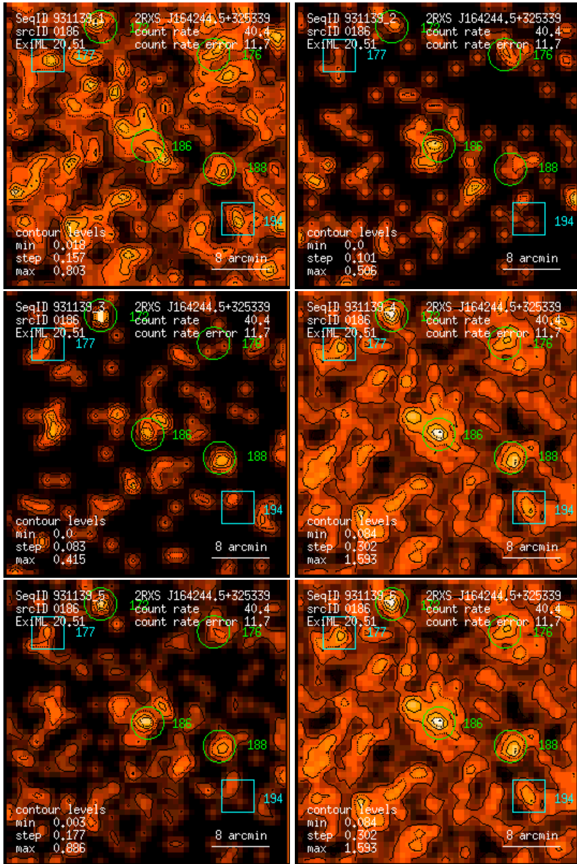
Figure 186: RASS 931139: detection 0186: band rate images, Gaussian filter: (1) PSPC channels 11 – 41, (2) 52 – 90, (3) 91 – 201, (4) 11 – 235, (5) 52 – 201, (6) 11 – 201. Broad band rates in counts/ks. Band rate contour levels in counts/ks/arcmin 2 .
