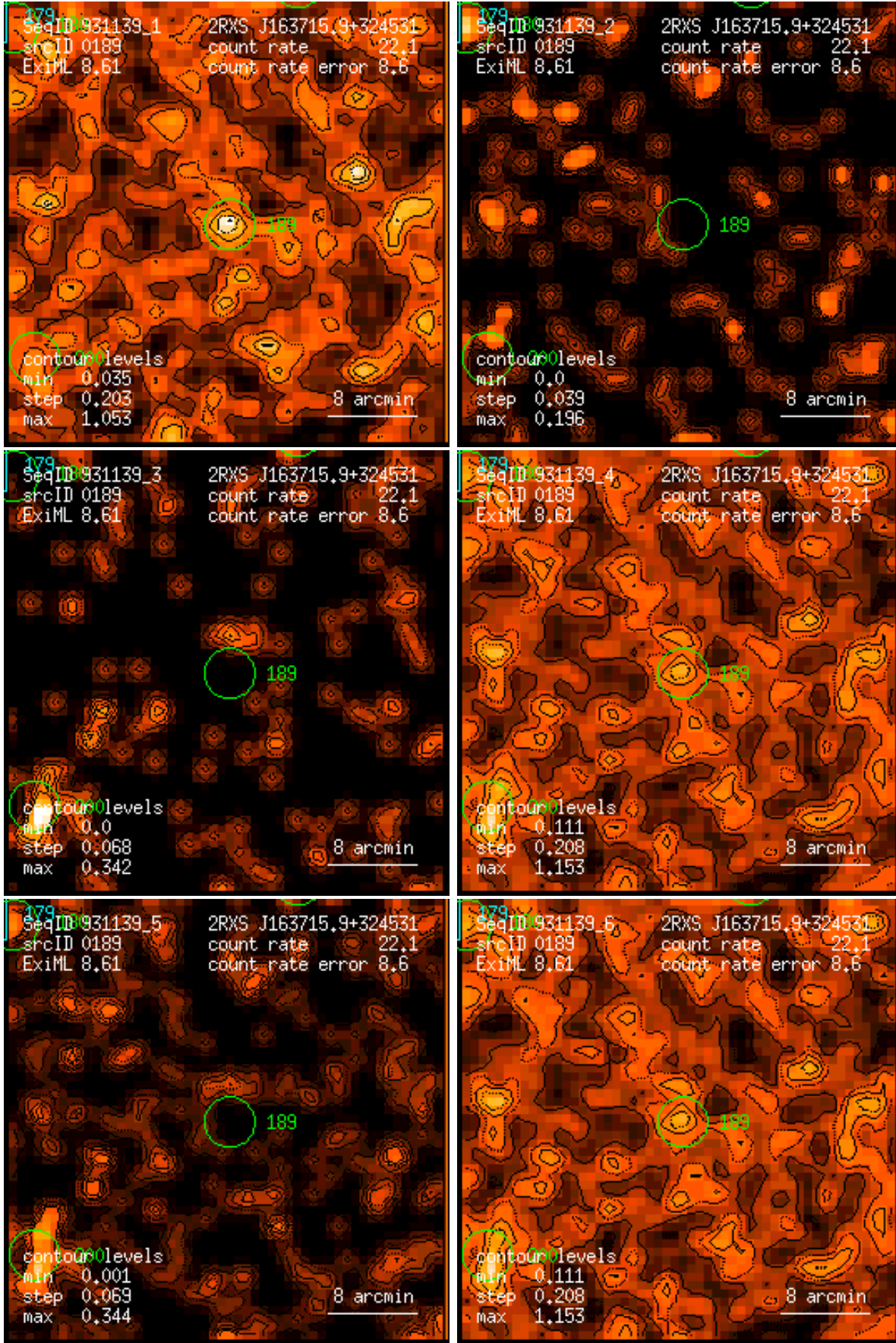
Figure 189: RASS 931139: detection 0189: band rate images, Gaussian filter: (1) PSPC channels 11 – 41, (2) 52 – 90, (3) 91 – 201, (4) 11 – 235, (5) 52 – 201, (6) 11 – 201. Broad band rates in counts/ks. Band rate contour levels in counts/ks/arcmin 2 .
