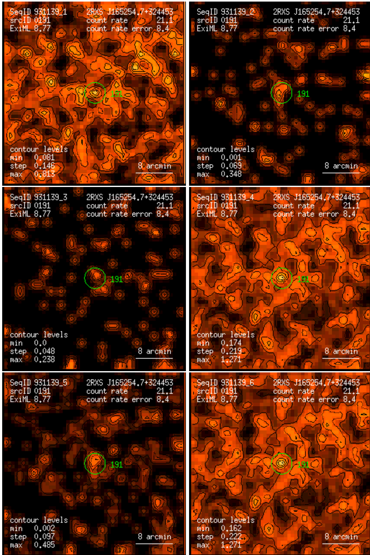
Figure 191: RASS 931139: detection 0191: band rate images, Gaussian filter: (1) PSPC channels 11 – 41, (2) 52 – 90, (3) 91 – 201, (4) 11 – 235, (5) 52 – 201, (6) 11 – 201. Broad band rates in counts/ks. Band rate contour levels in counts/ks/arcmin 2 .
