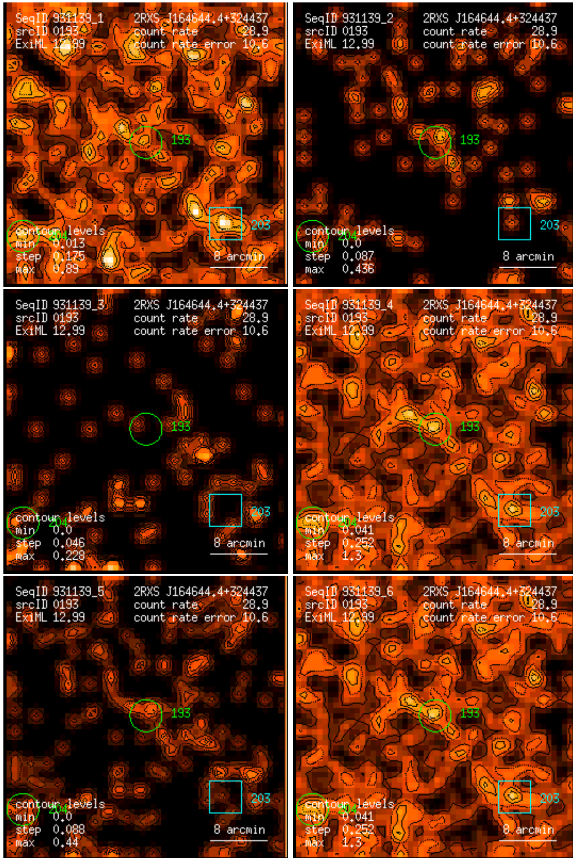
Figure 193: RASS 931139: detection 0193: band rate images, Gaussian filter: (1) PSPC channels 11 – 41, (2) 52 – 90, (3) 91 – 201, (4) 11 – 235, (5) 52 – 201, (6) 11 – 201. Broad band rates in counts/ks. Band rate contour levels in counts/ks/arcmin 2 .
