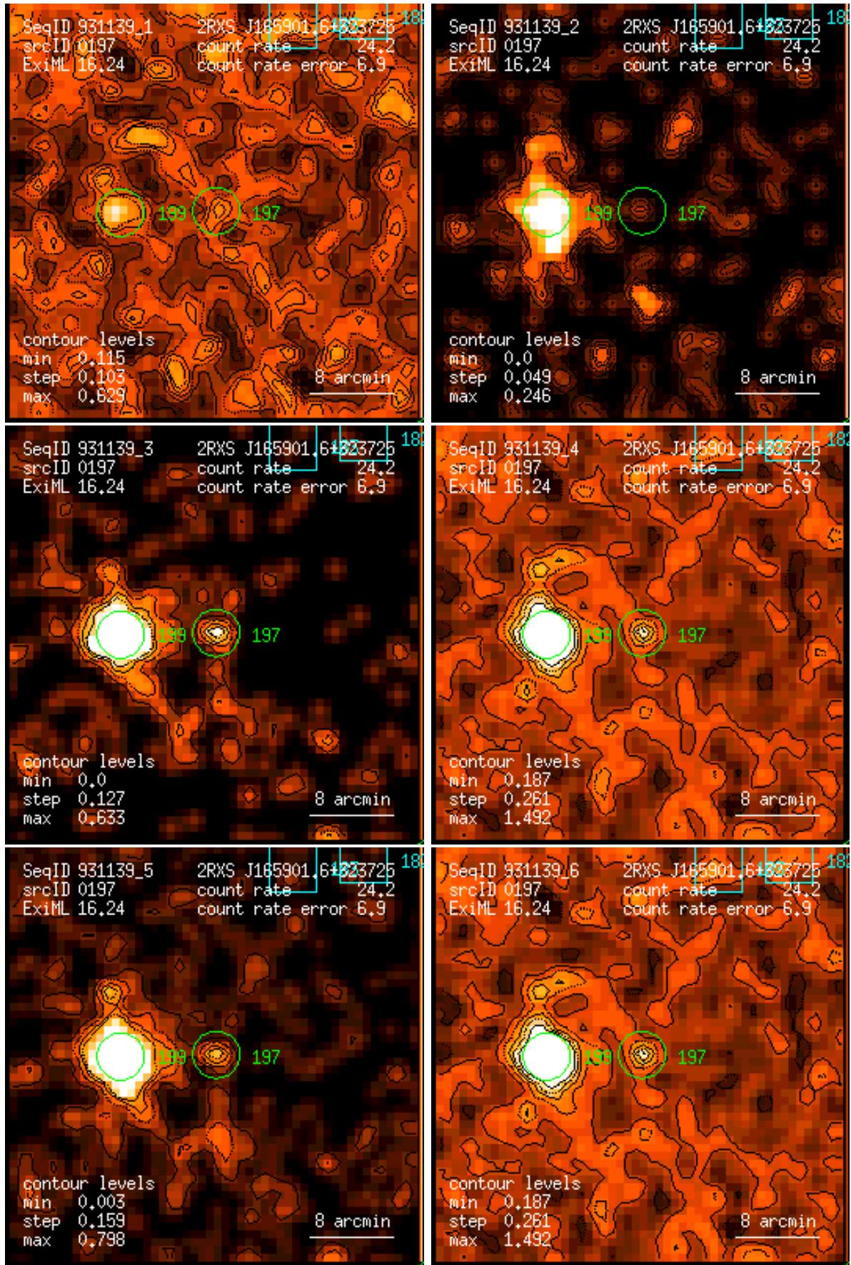
Figure 197: RASS 931139: detection 0197: band rate images, Gaussian filter: (1) PSPC channels 11 – 41, (2) 52 – 90, (3) 91 – 201, (4) 11 – 235, (5) 52 – 201, (6) 11 – 201. Broad band rates in counts/ks. Band rate contour levels in counts/ks/arcmin 2 .
