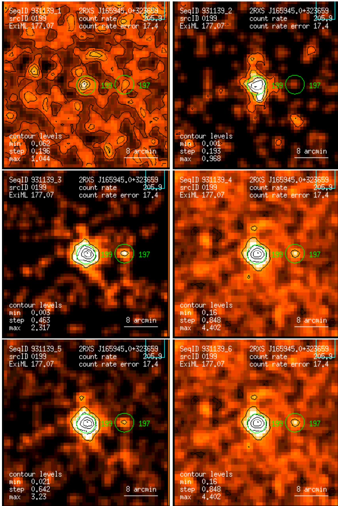
Figure 199: RASS 931139: detection 0199: band rate images, Gaussian filter: (1) PSPC channels 11 – 41, (2) 52 – 90, (3) 91 – 201, (4) 11 – 235, (5) 52 – 201, (6) 11 – 201. Broad band rates in counts/ks. Band rate contour levels in counts/ks/arcmin 2 .
