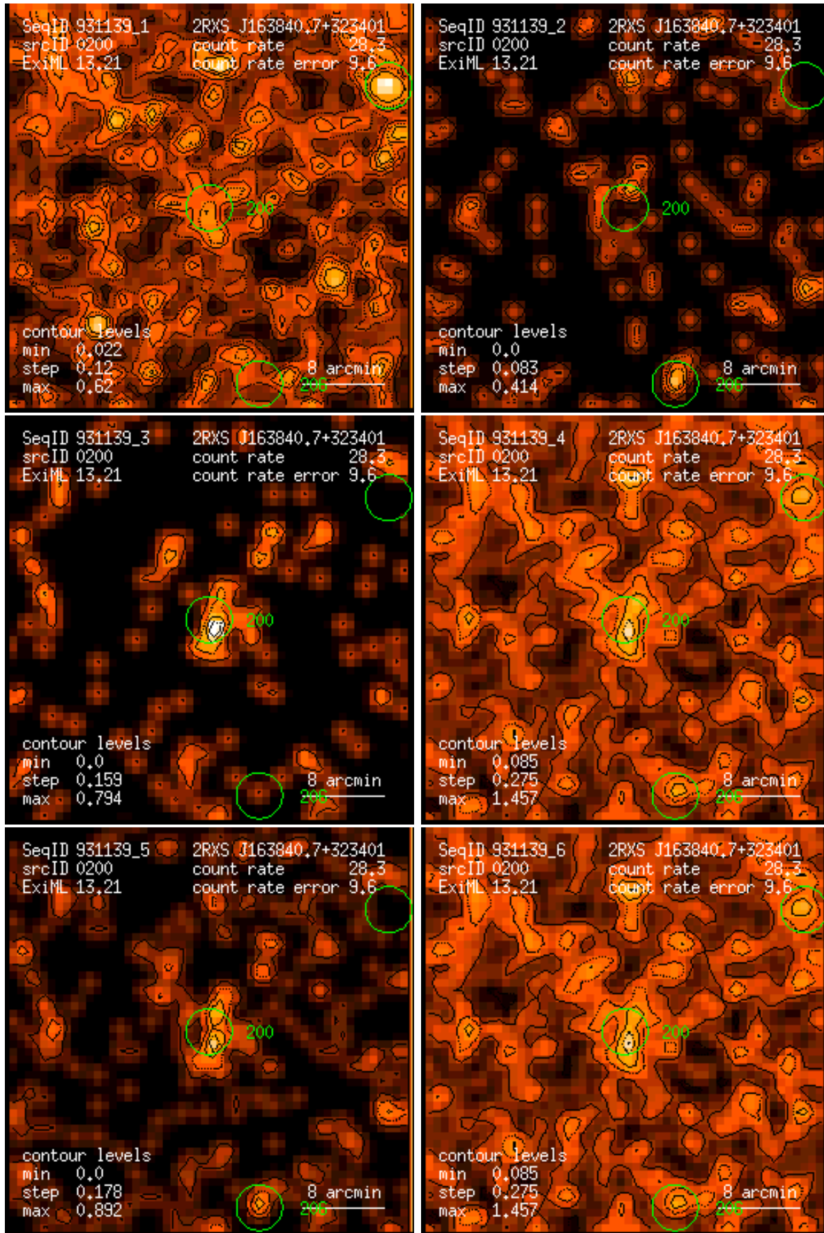
Figure 200: RASS 931139: detection 0200: band rate images, Gaussian filter: (1) PSPC channels 11 – 41, (2) 52 – 90, (3) 91 – 201, (4) 11 – 235, (5) 52 – 201, (6) 11 – 201. Broad band rates in counts/ks. Band rate contour levels in counts/ks/arcmin 2 .
