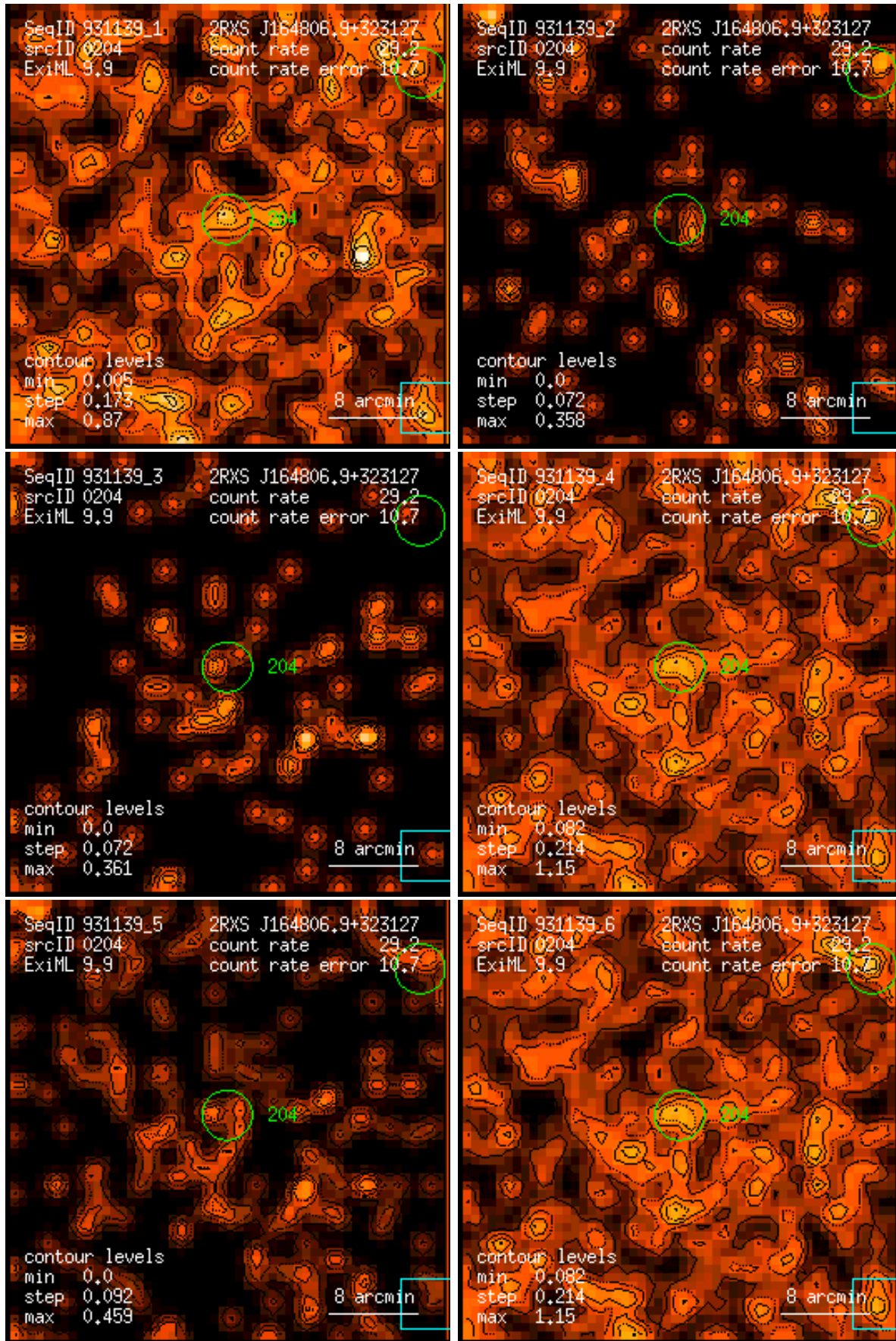
Figure 204: RASS 931139: detection 0204: band rate images, Gaussian filter: (1) PSPC channels 11 – 41, (2) 52 – 90, (3) 91 – 201, (4) 11 – 235, (5) 52 – 201, (6) 11 – 201. Broad band rates in counts/ks. Band rate contour levels in counts/ks/arcmin 2 .
