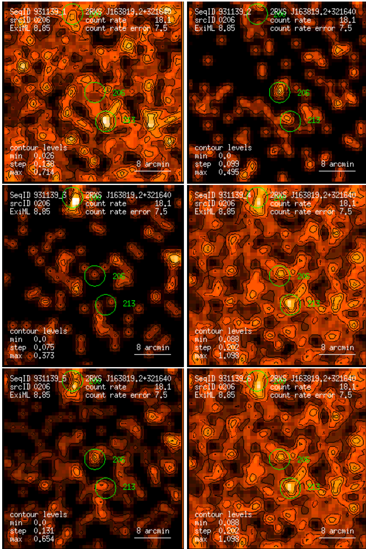
Figure 206: RASS 931139: detection 0206: band rate images, Gaussian filter: (1) PSPC channels 11 – 41, (2) 52 – 90, (3) 91 – 201, (4) 11 – 235, (5) 52 – 201, (6) 11 – 201. Broad band rates in counts/ks. Band rate contour levels in counts/ks/arcmin 2 .
