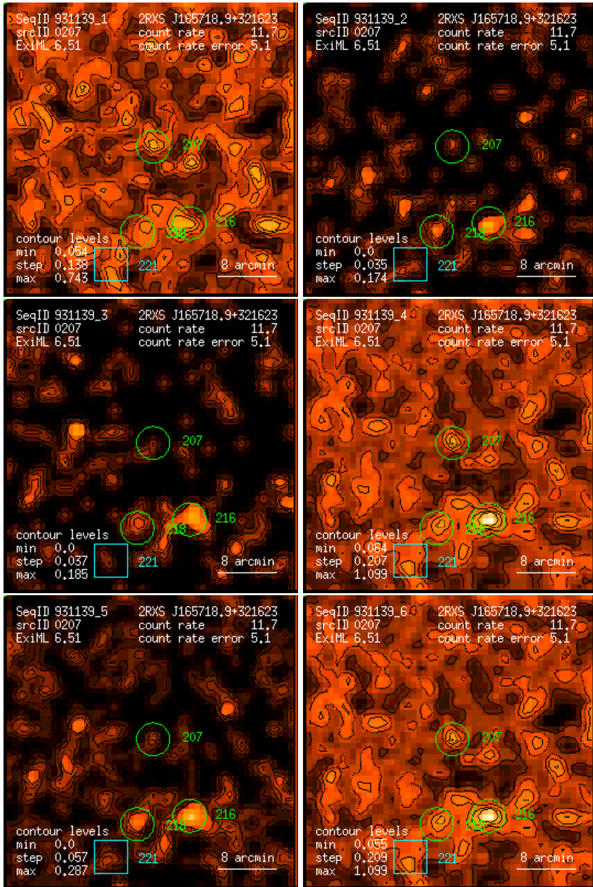
Figure 207: RASS 931139: detection 0207: band rate images, Gaussian filter: (1) PSPC channels 11 – 41, (2) 52 – 90, (3) 91 – 201, (4) 11 – 235, (5) 52 – 201, (6) 11 – 201. Broad band rates in counts/ks. Band rate contour levels in counts/ks/arcmin 2 .
