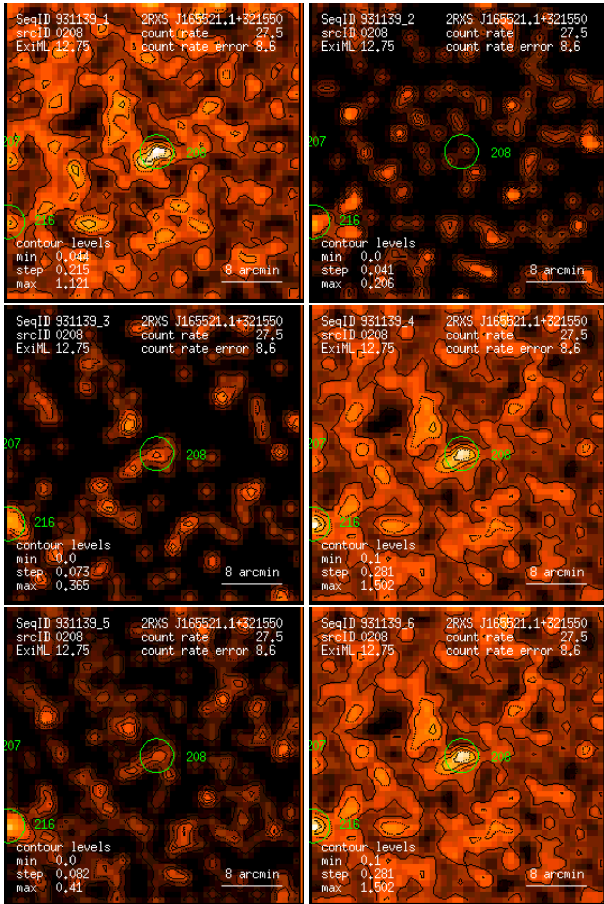
Figure 208: RASS 931139: detection 0208: band rate images, Gaussian filter: (1) PSPC channels 11 – 41, (2) 52 – 90, (3) 91 – 201, (4) 11 – 235, (5) 52 – 201, (6) 11 – 201. Broad band rates in counts/ks. Band rate contour levels in counts/ks/arcmin 2 .
