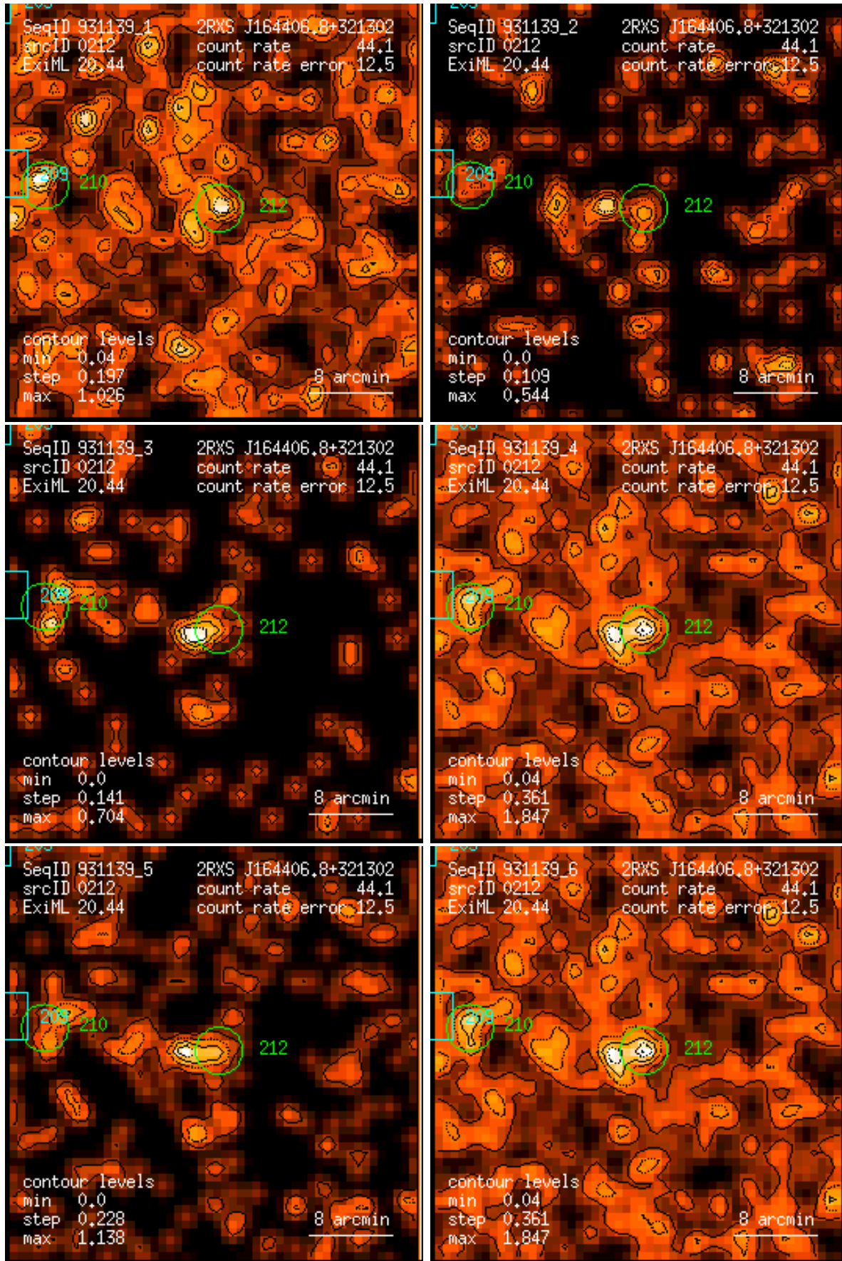
Figure 212: RASS 931139: detection 0212: band rate images, Gaussian filter: (1) PSPC channels 11 – 41, (2) 52 – 90, (3) 91 – 201, (4) 11 – 235, (5) 52 – 201, (6) 11 – 201. Broad band rates in counts/ks. Band rate contour levels in counts/ks/arcmin 2 .
