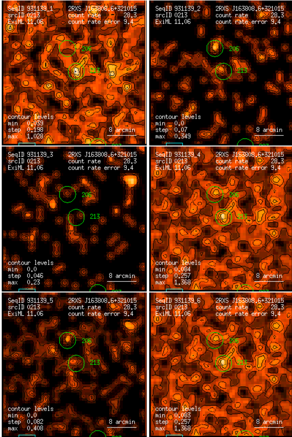
Figure 213: RASS 931139: detection 0213: band rate images, Gaussian filter: (1) PSPC channels 11 – 41, (2) 52 – 90, (3) 91 – 201, (4) 11 – 235, (5) 52 – 201, (6) 11 – 201. Broad band rates in counts/ks. Band rate contour levels in counts/ks/arcmin 2 .
