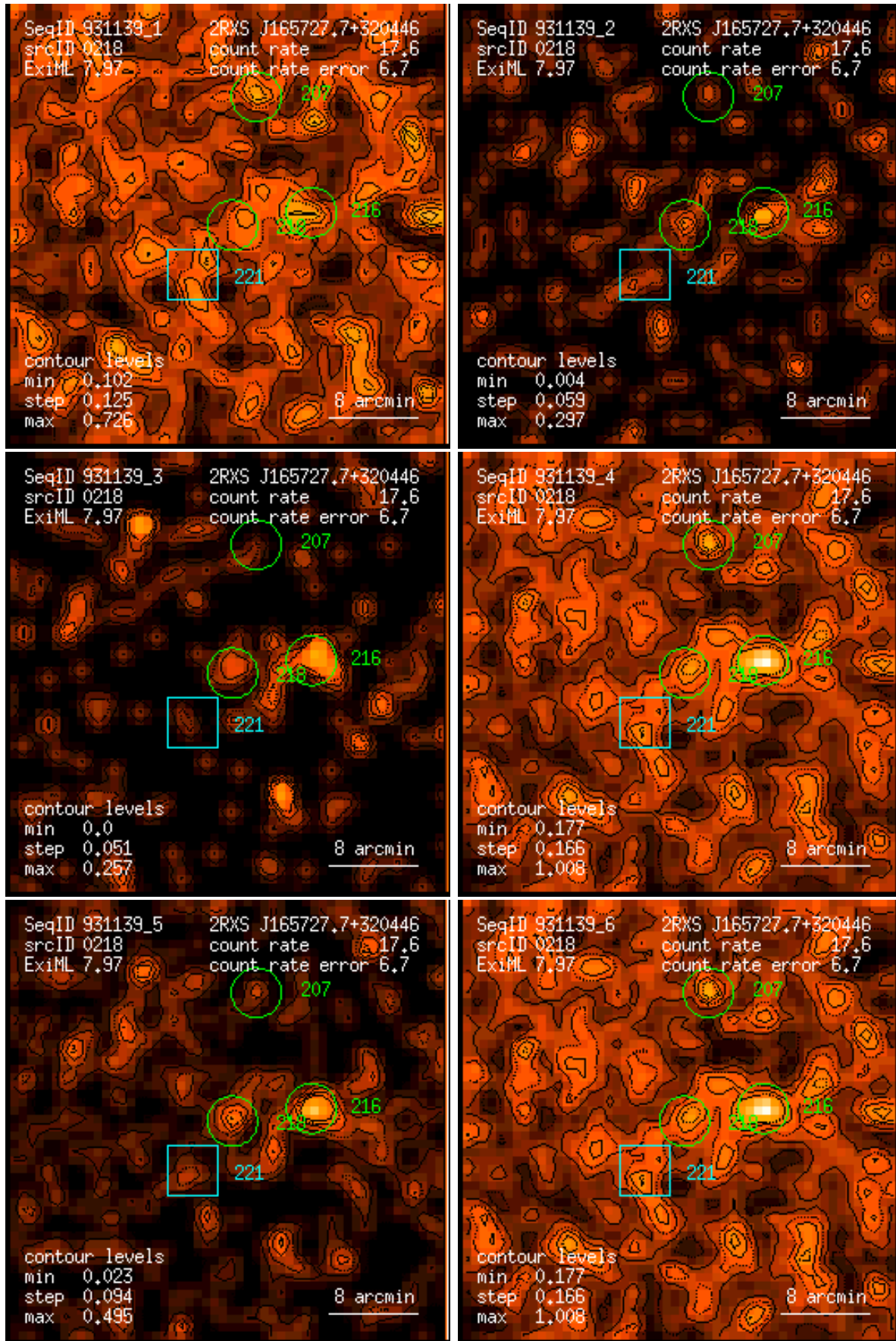
Figure 218: RASS 931139: detection 0218: band rate images, Gaussian filter: (1) PSPC channels 11 – 41, (2) 52 – 90, (3) 91 – 201, (4) 11 – 235, (5) 52 – 201, (6) 11 – 201. Broad band rates in counts/ks. Band rate contour levels in counts/ks/arcmin 2 .
