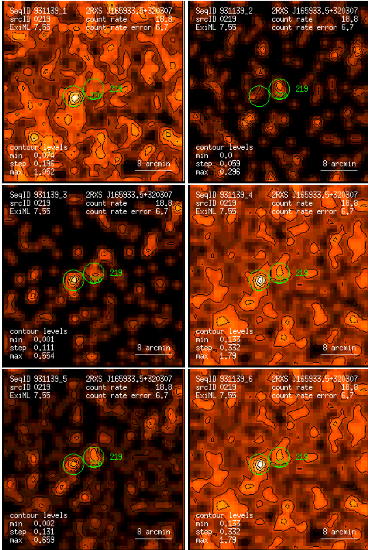
Figure 219: RASS 931139: detection 0219: band rate images, Gaussian filter: (1) PSPC channels 11 – 41, (2) 52 – 90, (3) 91 – 201, (4) 11 – 235, (5) 52 – 201, (6) 11 – 201. Broad band rates in counts/ks. Band rate contour levels in counts/ks/arcmin 2 .
