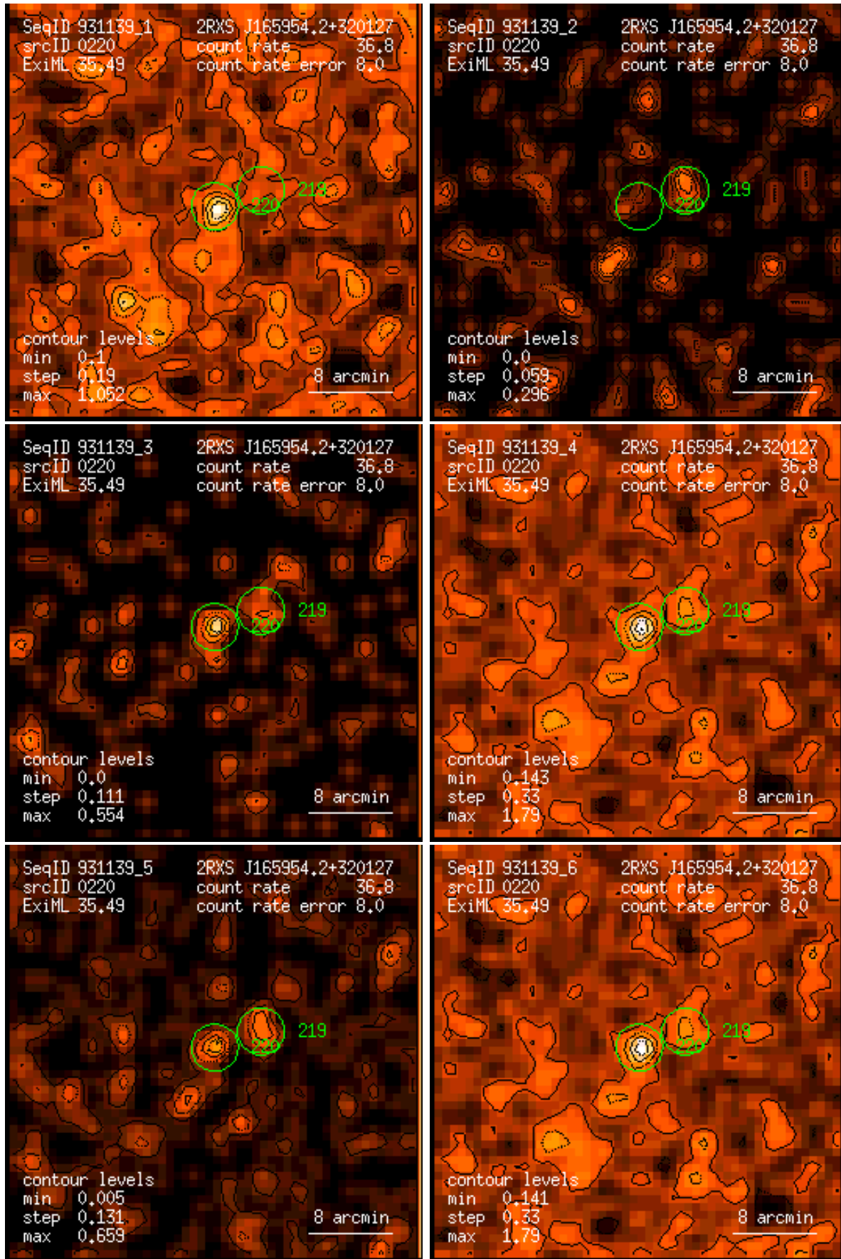
Figure 220: RASS 931139: detection 0220: band rate images, Gaussian filter: (1) PSPC channels 11 – 41, (2) 52 – 90, (3) 91 – 201, (4) 11 – 235, (5) 52 – 201, (6) 11 – 201. Broad band rates in counts/ks. Band rate contour levels in counts/ks/arcmin 2 .
