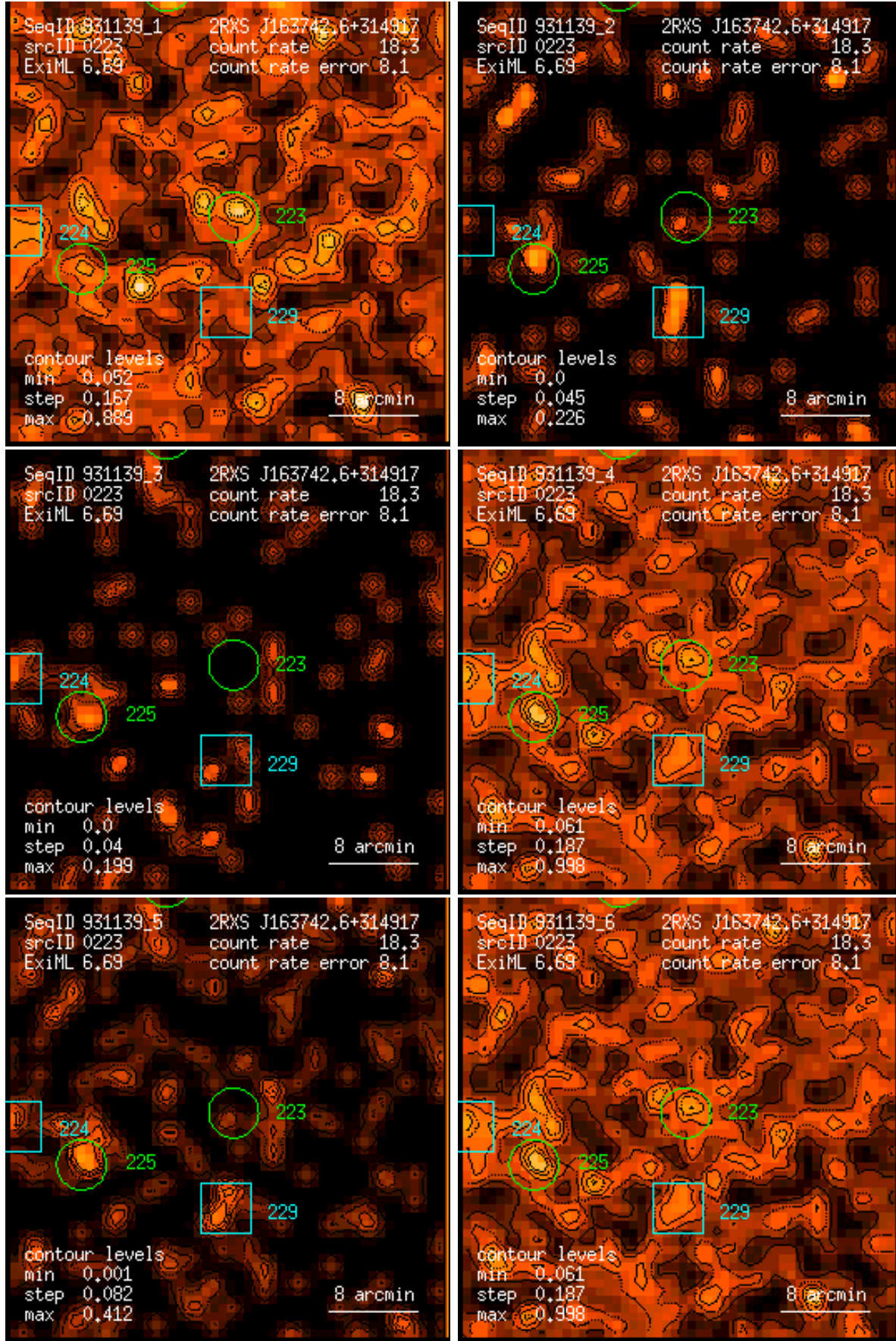
Figure 223: RASS 931139: detection 0223: band rate images, Gaussian filter: (1) PSPC channels 11 – 41, (2) 52 – 90, (3) 91 – 201, (4) 11 – 235, (5) 52 – 201, (6) 11 – 201. Broad band rates in counts/ks. Band rate contour levels in counts/ks/arcmin 2 .
