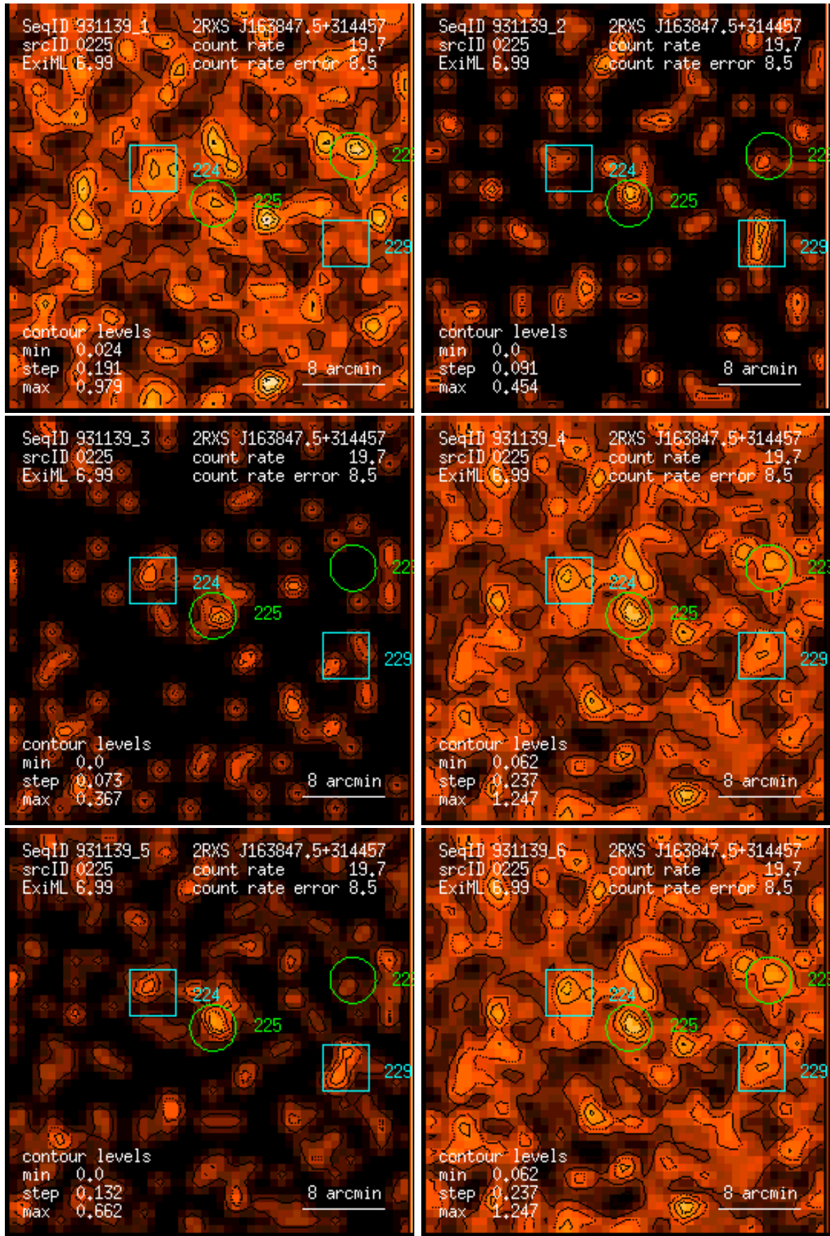
Figure 225: RASS 931139: detection 0225: band rate images, Gaussian filter: (1) PSPC channels 11 – 41, (2) 52 – 90, (3) 91 – 201, (4) 11 – 235, (5) 52 – 201, (6) 11 – 201. Broad band rates in counts/ks. Band rate contour levels in counts/ks/arcmin 2 .
