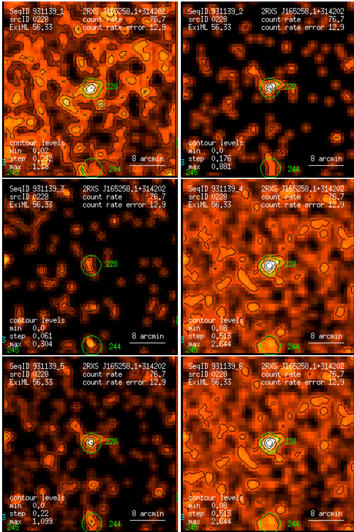
Figure 228: RASS 931139: detection 0228: band rate images, Gaussian filter: (1) PSPC channels 11 – 41, (2) 52 – 90, (3) 91 – 201, (4) 11 – 235, (5) 52 – 201, (6) 11 – 201. Broad band rates in counts/ks. Band rate contour levels in counts/ks/arcmin 2 .
