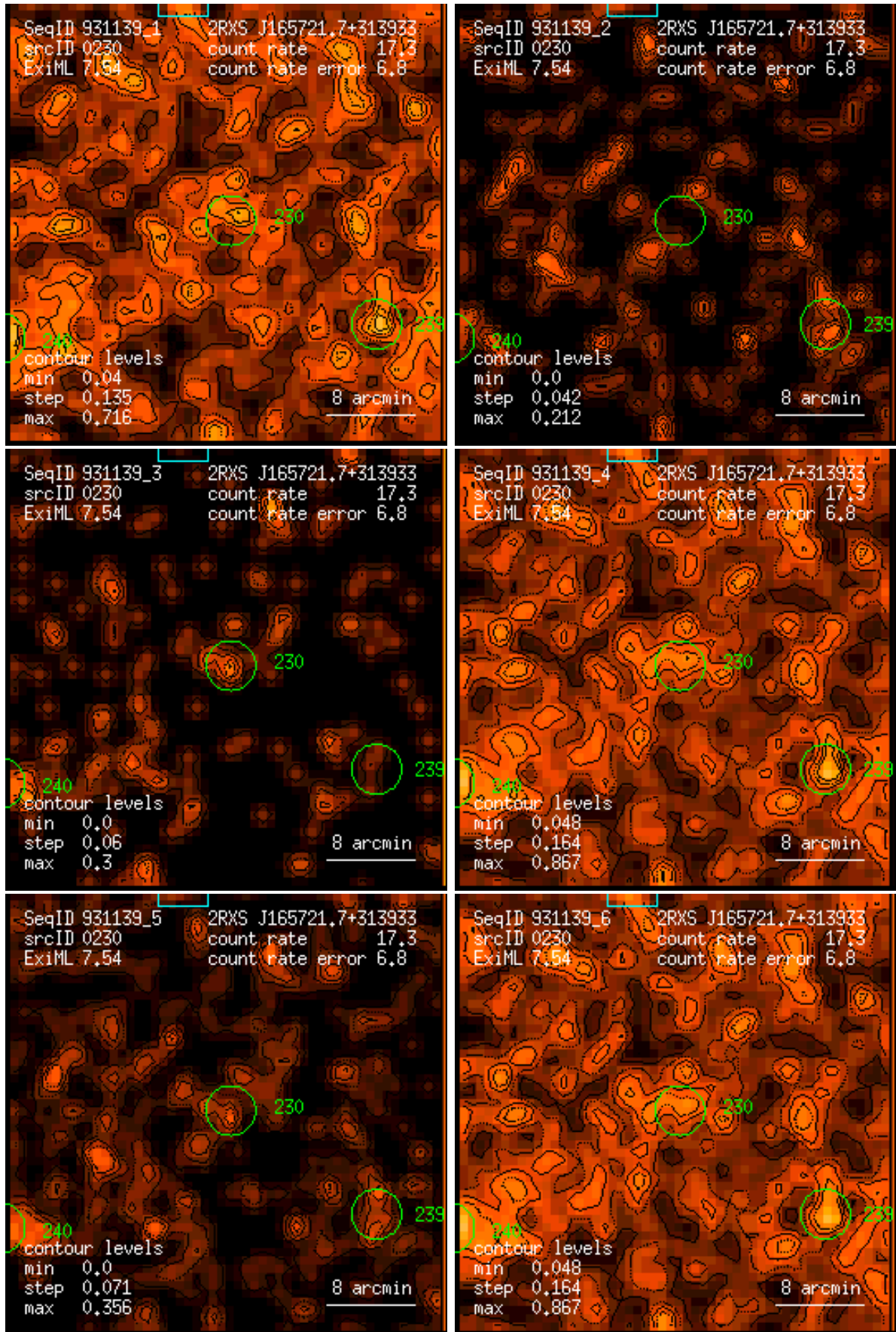
Figure 230: RASS 931139: detection 0230: band rate images, Gaussian filter: (1) PSPC channels 11 – 41, (2) 52 – 90, (3) 91 – 201, (4) 11 – 235, (5) 52 – 201, (6) 11 – 201. Broad band rates in counts/ks. Band rate contour levels in counts/ks/arcmin 2 .
