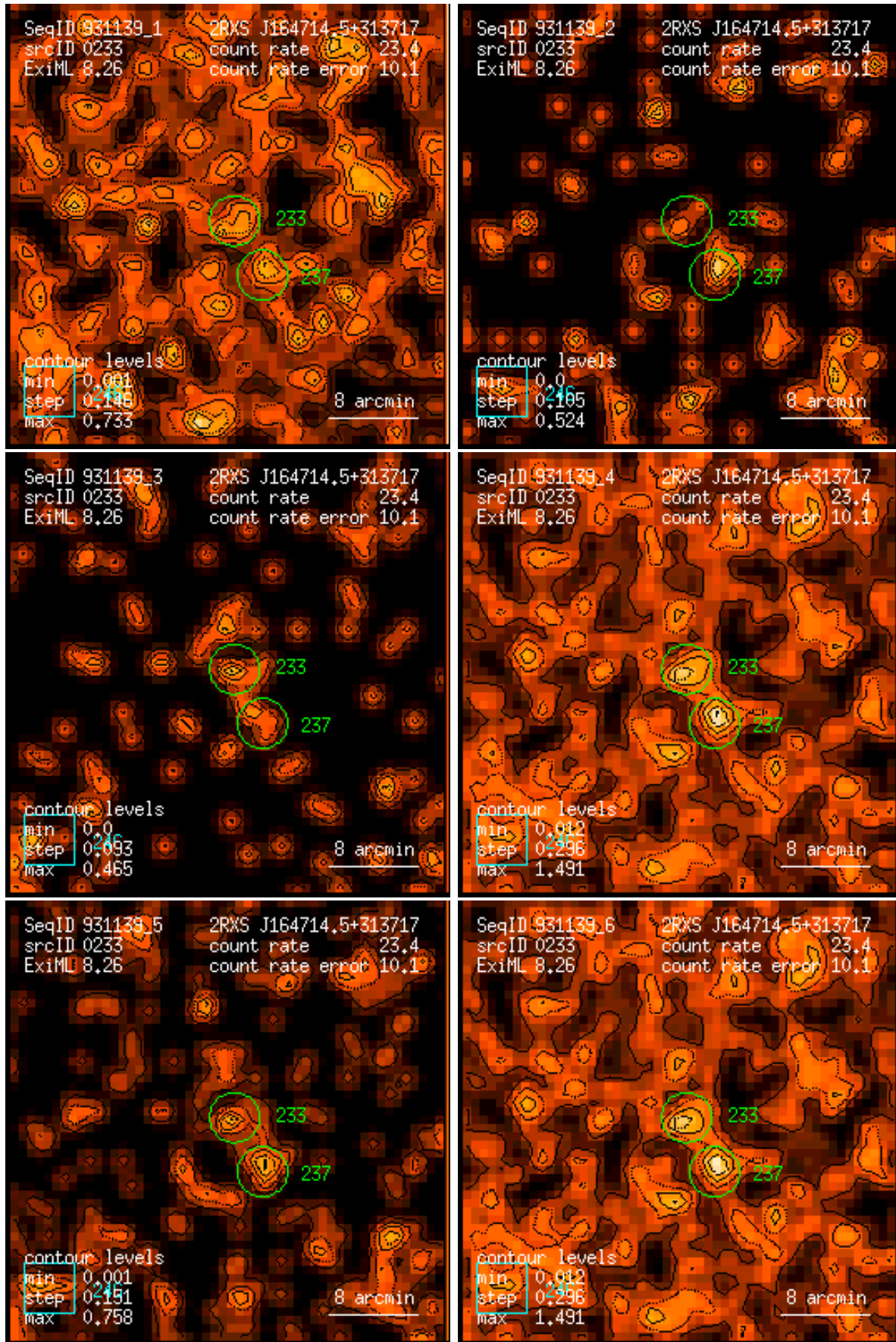
Figure 233: RASS 931139: detection 0233: band rate images, Gaussian filter: (1) PSPC channels 11 – 41, (2) 52 – 90, (3) 91 – 201, (4) 11 – 235, (5) 52 – 201, (6) 11 – 201. Broad band rates in counts/ks. Band rate contour levels in counts/ks/arcmin 2 .
