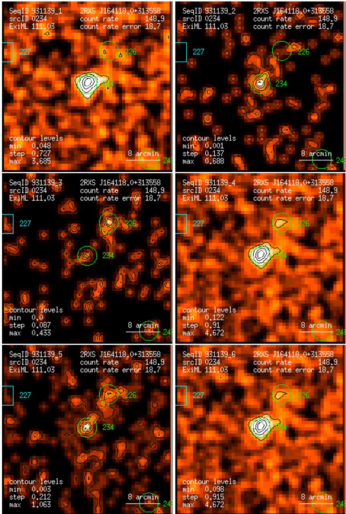
Figure 234: RASS 931139: detection 0234: band rate images, Gaussian filter: (1) PSPC channels 11 – 41, (2) 52 – 90, (3) 91 – 201, (4) 11 – 235, (5) 52 – 201, (6) 11 – 201. Broad band rates in counts/ks. Band rate contour levels in counts/ks/arcmin 2 .
