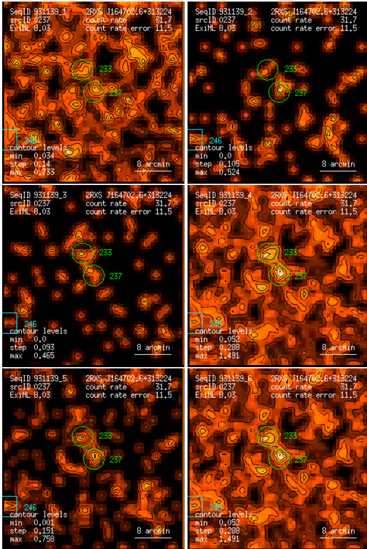
Figure 237: RASS 931139: detection 0237: band rate images, Gaussian filter: (1) PSPC channels 11 – 41, (2) 52 – 90, (3) 91 – 201, (4) 11 – 235, (5) 52 – 201, (6) 11 – 201. Broad band rates in counts/ks. Band rate contour levels in counts/ks/arcmin 2 .
